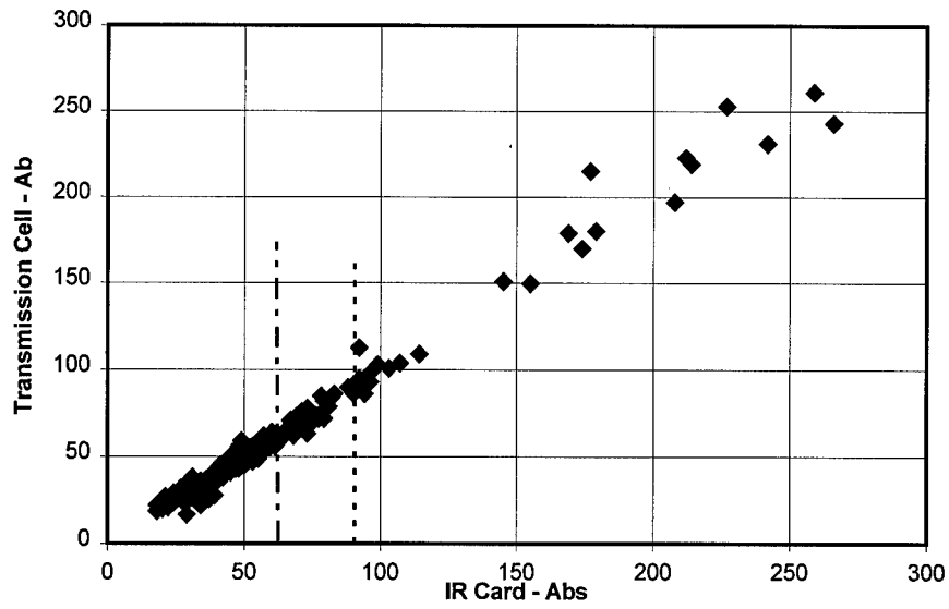
Figure 8: Comparison of Lubricant Breakdown (region I) Data Breakdown I measurement coefficient of correlation = 0.99
