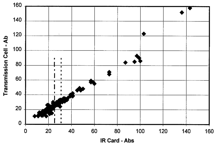
Figure 9: Comparison of Lubricant Breakdown (region II) Data Breakdown II measurement coefficient of correlation = 0.99
