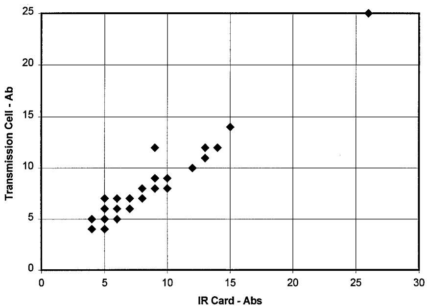
Figure 4: Comparison of Nitration Data Nitration measurement coefficient of correlation = 0.97
