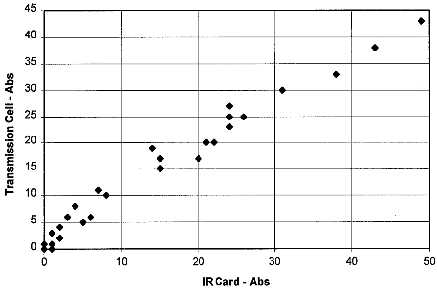
Figure 2: Comparison of Soot Data Soot measurement coefficient of correlation = 0.99
