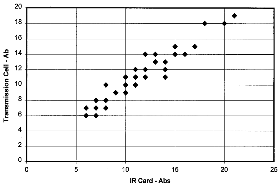
Figure 3: Comparison of Oxidation Data Oxidation measurement coefficient of correlation = 0.97
