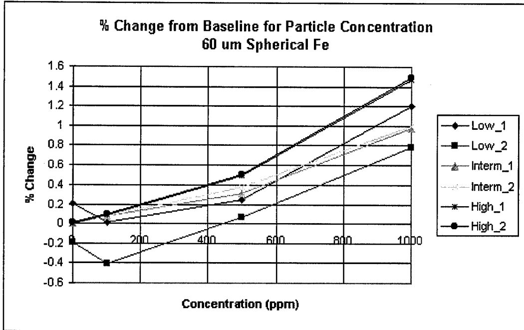
Figure 4: Ferrous Particle Response in Navigator v1.0
