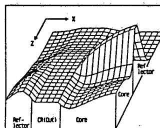
Fig. 4. Thermal neutron flux distribution on the XZ plane based on diffusion calculation (S8) with the absorber rods completely removed.
