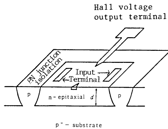
Figure 1. Hall Element Manufactured by a Bipolar Process
