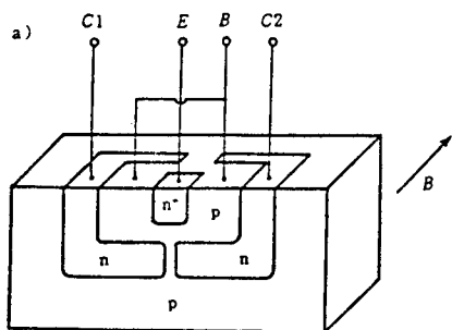
Figure 7. Hudson's Magnetic Transistor
