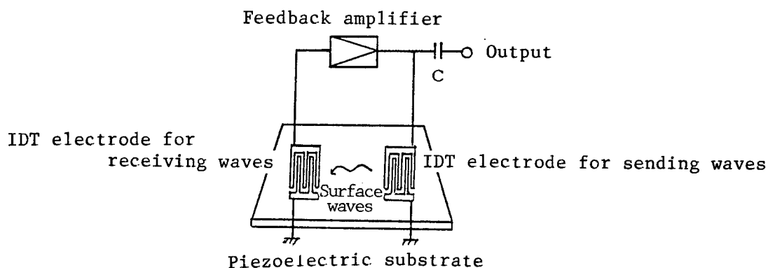
Figure 6. Structure of an Elastic Surface-Wave Temperature Sensor 8)
