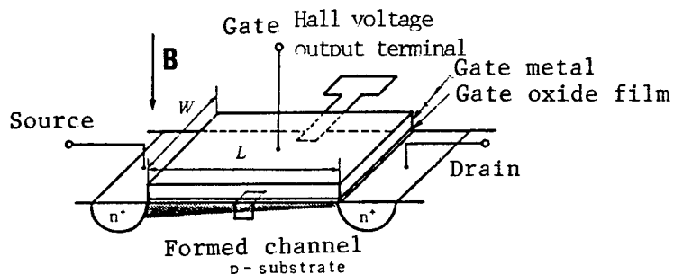
Figure 6. An MOS Hall Element
