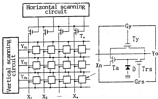
Figure 5. AMI Image Sensor 16)
