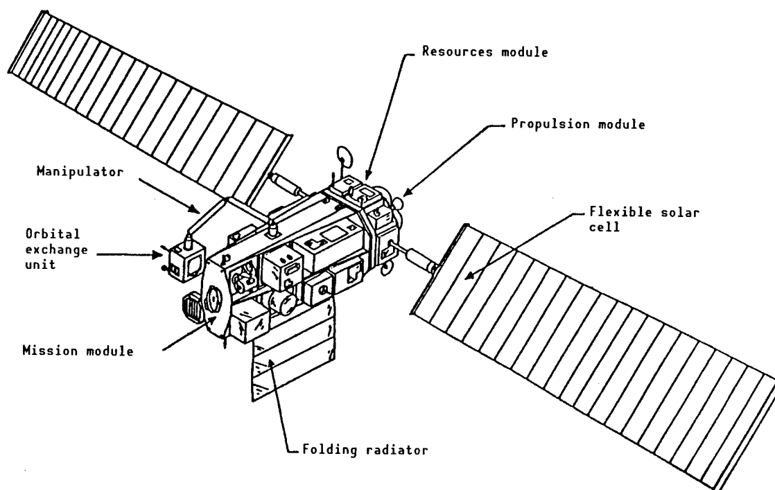
Figure 4. Conceptual Diagram of Application Technology Platform
