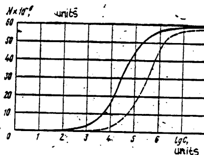
Figure 2. Dependence of Annual Productivity of Automatic Press on Series of Parts To Be Die-Forged. — T = 10 min; - - - T = 90 min
