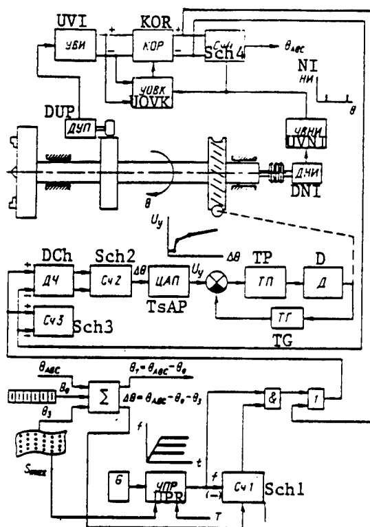
Block Diagram of the "Radian" System
