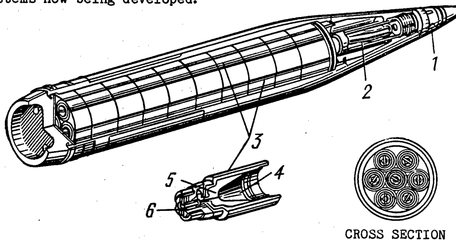
Fig. 5. West German RB-63 155mm cluster shell: 1--remote detonator; 2--bursting charge; 3--hollow-charge fragmentation elements; 4--copper lining of the hollow charge; 5--explosive; 6--fuse.
