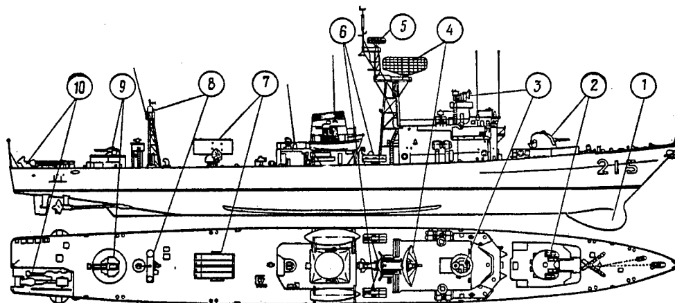
Fig. 3. Japanese Tikugo-class frigate: 1--Keel low-frequency type-66 sonar (QQS-3A); 2--76mm type-68 paired gun (Mk33); 3--fire-control radar antenna; 4--OPS-14 airborne target-detection radar antenna; 5--OPS-17 surface-target detection radar antenna; 6--324mm type-68 three-tube torpedo apparatus (Mk32); 7--eight-charge type-74 ASROC launcher (Mk16); 8--NOLR-1B (NOLR-5 for the DE219 Ivasa) radio and ECM station antennas; 9--40mm paired Mk1 guns; 10--AN/SQS-35 variable-depth towed sonar (except for DE216 Awaji, DE217 Mikuma, DE221 Niyodo, DE222 Teshio and DE225 Noshiro)
