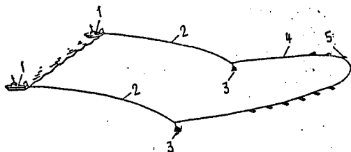
Fig 2. Towing Schematic for the WS Mk9 Paired Deepwater Contact Sweep.
