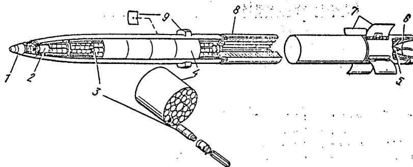
Fig 1. Free-Flight Rocket with Shaped-Charge Fragmentation Warhead.
