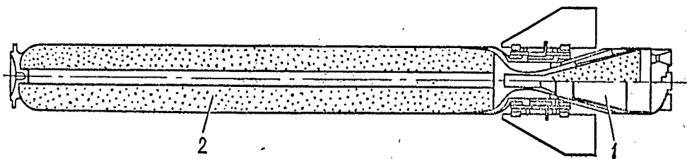
Fig 2. Mistral Propulsion System.
