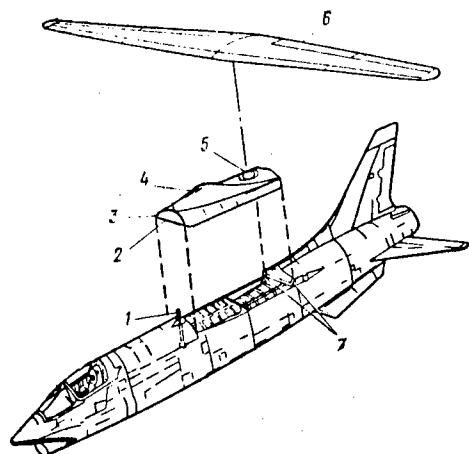
Figure 4. Modified components and assemblies of the F-8 experimental aircraft: 1 -- gear for changing established wing attack angle; 2 -- attachment mount for the gear for changing established wing attack angle; 3 -- wing supporting structure; 4 -- cowling; 5 -- hinged wing attachment mount; 6 -- "slanted" wing; 7 -- rear attachment mounts of wing support structure.
