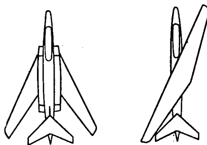
Figure 3. Fighter diagrams according to Rockwell International design studies: left -- with variable swept back wing; right -- with slanted variable sweep wing.
