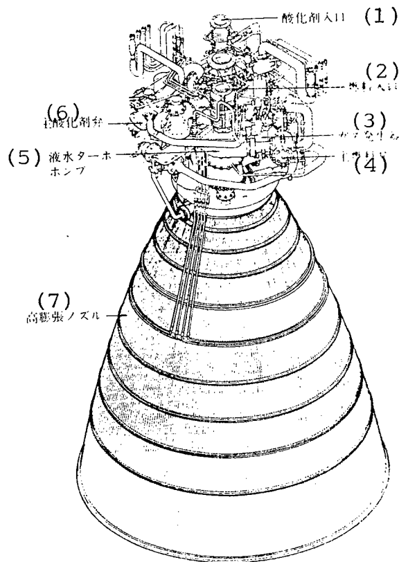
Figure 2 H-I Second-Stage Engine
