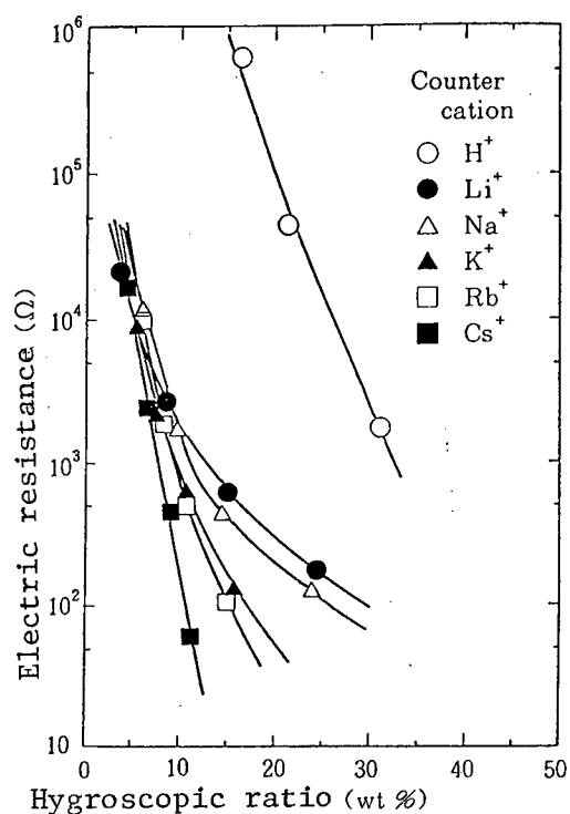
Figure 10. Relation Between Electric Resistance and Hygroscopic Ratio of Copolymer of Styrene Sulfonic Acid and Styrene, Each Having Different Counter Ion Group
