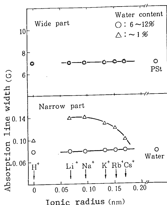
Figure 9. Absorption Line Width of NMR When Copolymer of Styrene Sulfonic Acid and Styrene, Different in Counter Ion Group, Has Undergone Moisture Absorption
