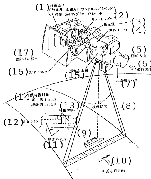
Figure 2 VTIR Configuration
