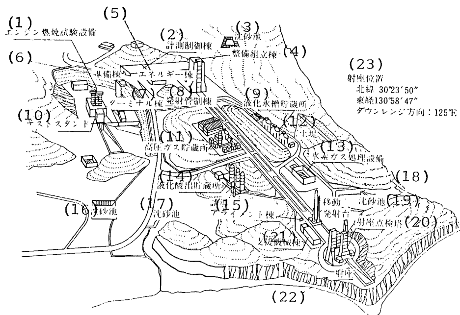
Figure 6 H-II Rocket Launch Complex Layout
