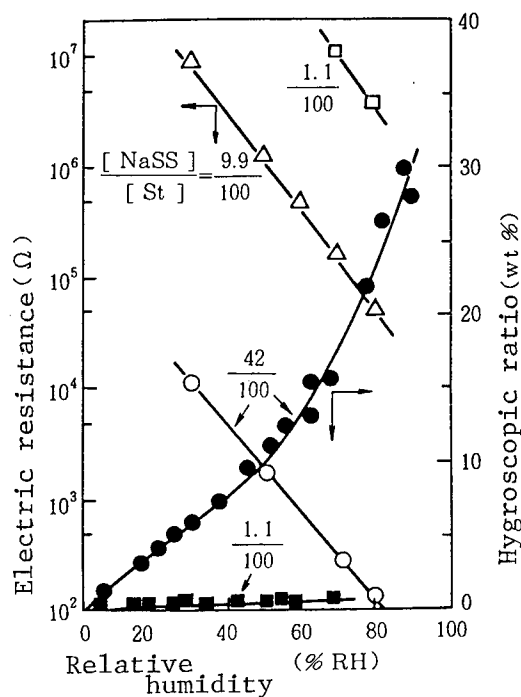
Figure 2. Humidity Sensitive Characteristic and Hygroscopic Isotherm of Poly (NaSS-co-St)
