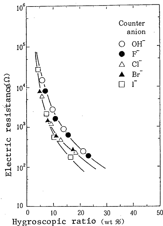
Figure 11. Relation Between Electric Resistance and Hygroscopic Ratio of Copolymer of METMA and MMA, Each Having Different Counter Ion
