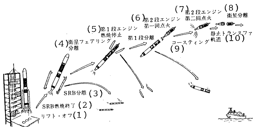
Figure 5 Flight Sequence
