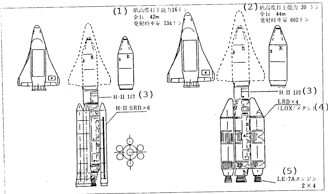
Figure 9 Examples of Enhanced H-II Vehicles
