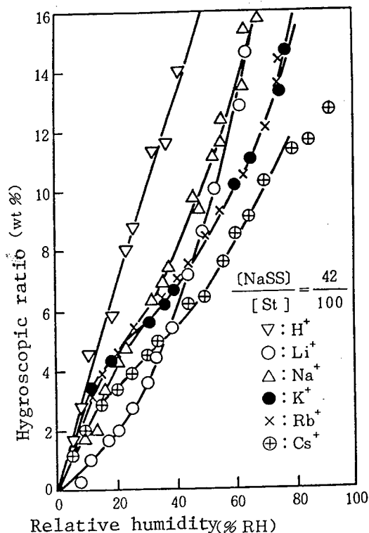
Figure 5. Hygroscopic Isothermal Curves of Copolymer of Styrene Sulfonic Acid and Styrene, Having Different Counter Ions
