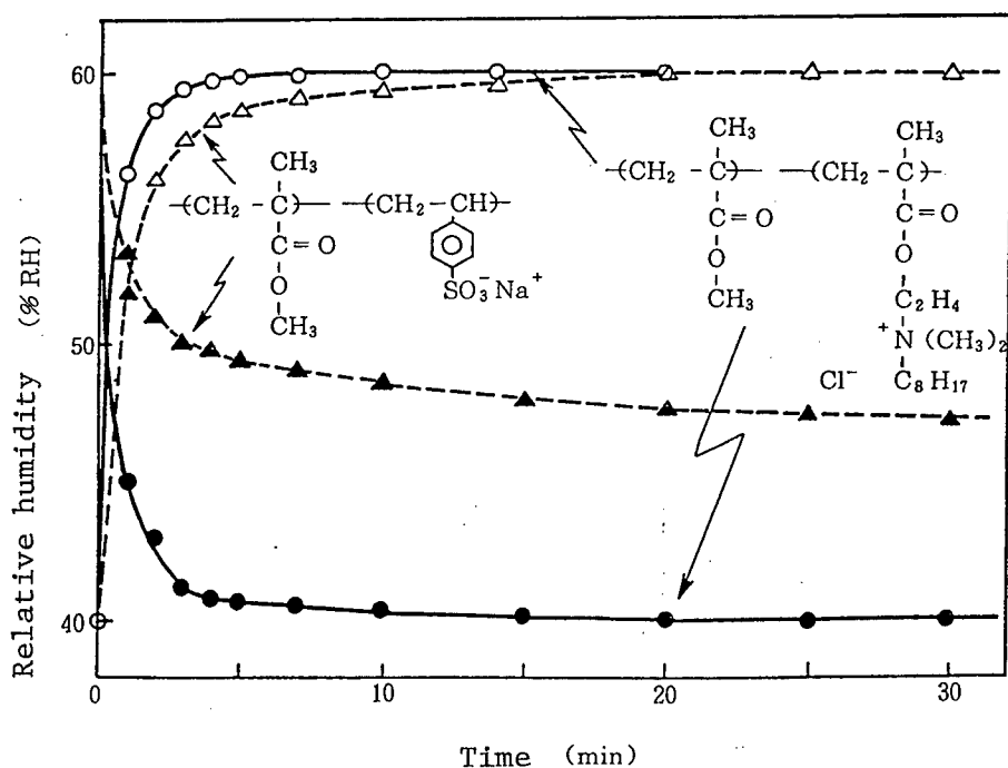
Figure 7. Comparison of Responsibility Between Humidity Sensors With Different Humidity Sensitive Materials
