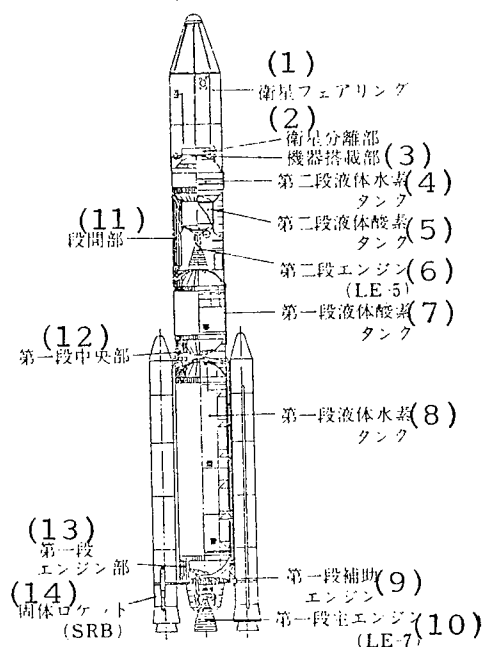
Figure 3 H-II Rocket
