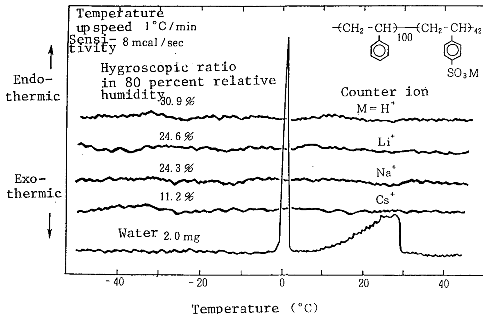
Figure 8. DSC Chart of Hygroscopic Water in Copolymer Having Undergone Moisture Absorption in Relative Humidity of 80 Percent
