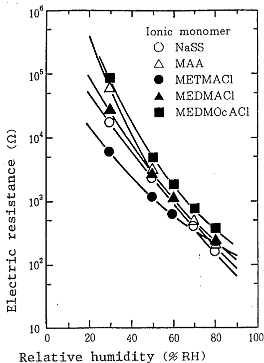
Figure 4. Influence of Type of Ionic Monomers on Humidity Sensitive Characteristic of Polymethyl Methacrylate Copolymer
