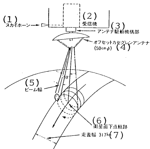
Figure 3 MSR Configuration
