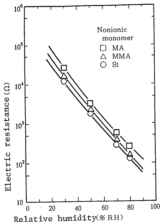
Figure 3. Influence of Type of Nonionic Monomers on Humidity Sensitive Characteristic of Polystyrene-Sulfonate Copolymer
