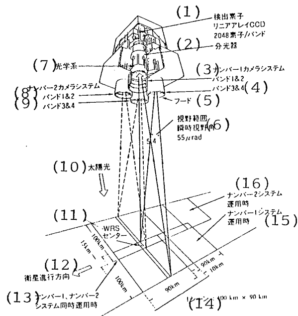
Figure 1 MESSR Configuration
