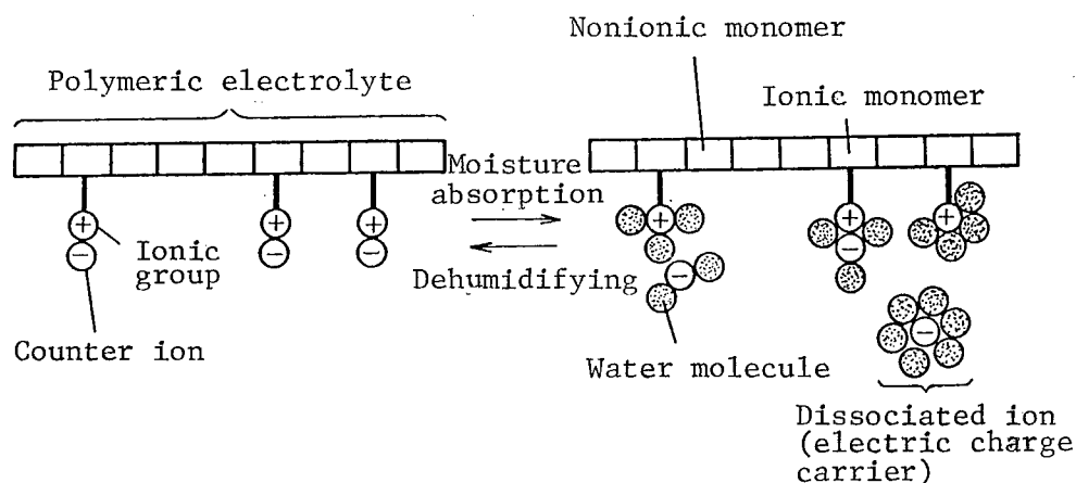
Figure 1. Operational Principle of Humidity Sensor Using Ionic Conductive Polymer (Conductivity generating mechanism)
