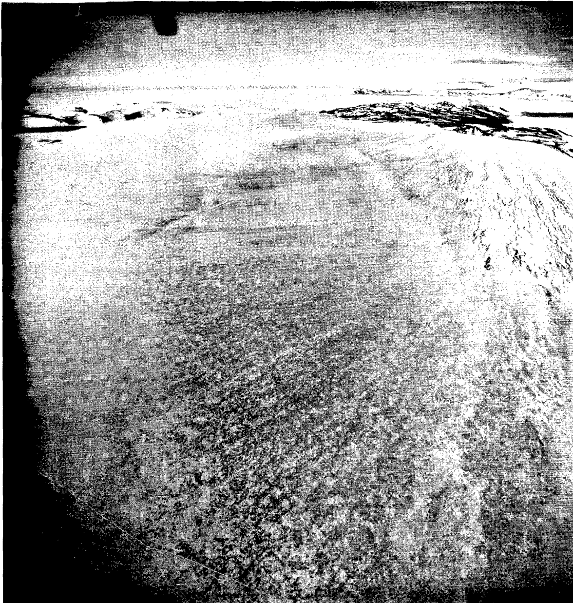
b. Photo taken in late January 1970 looking south (U.S. Navy for U.S. Geological Survey). Note airstrips of Outer Williams Field located just outside the zone of accumulation.
