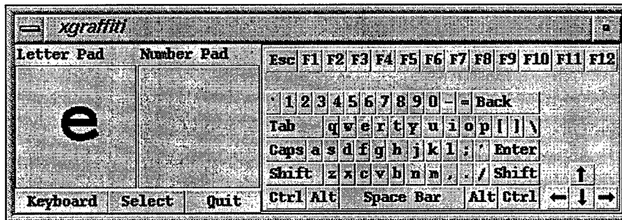
Figure 4-28 XGraffiti
