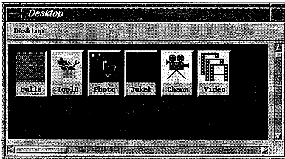
Figure 4-7 CSCW Desktop
