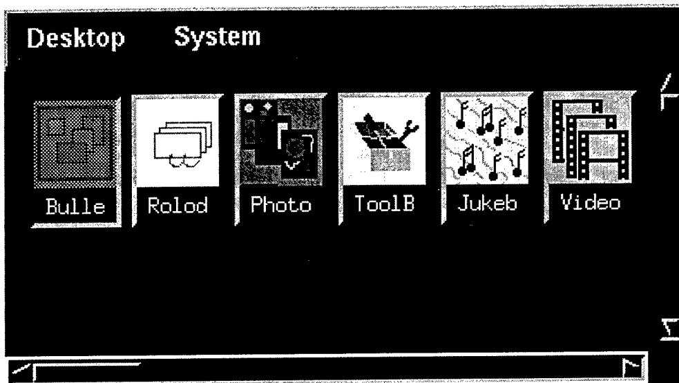
Figure 3: MultiTalk Desktop
