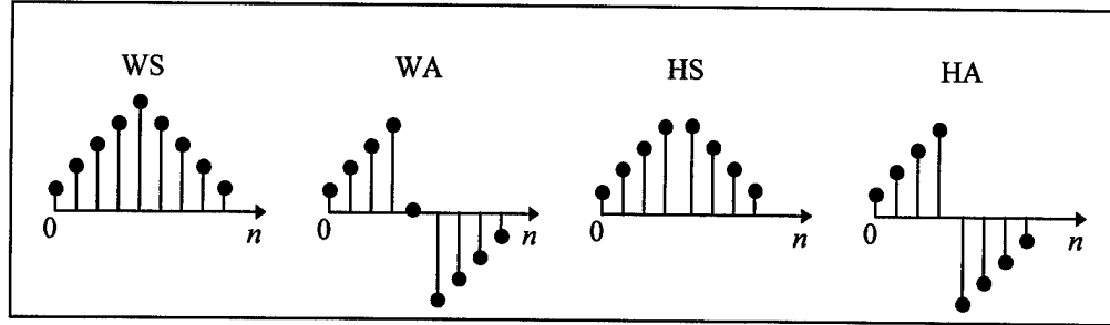
Figure 2. Four Ways to Symmetrically Extend a Finite Sequence [34]
