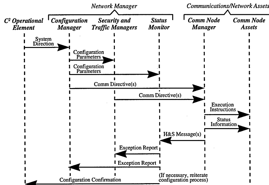
Figure 4-23a. Operational Event/Trace Description (OV-6c) — Communications Net Management Example
