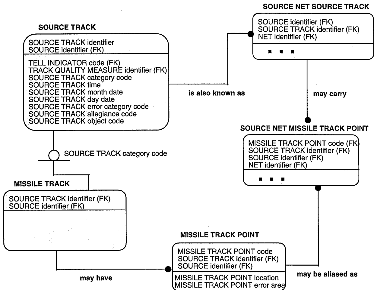
Figure 4-18a. Operational Rules Model (OV-6a) -- BMD Active Defense Example Employing a Logical Data Model
