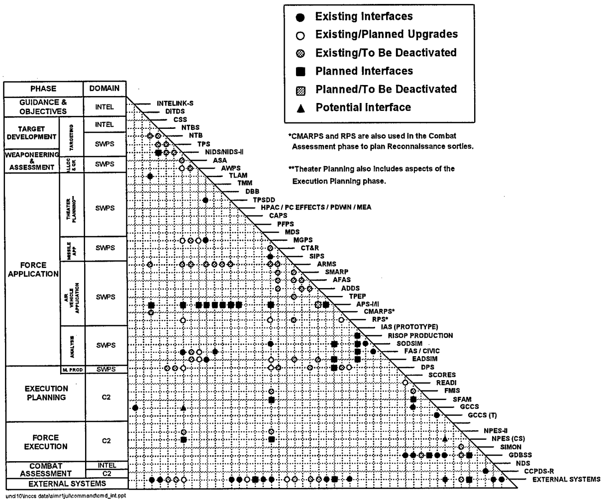
Figure 4-26b. Systems 2 Matrix (SV-3) -- USSTRATCOM Functional Interfaces Example
