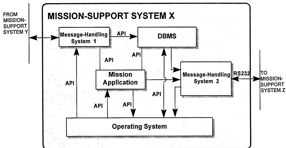
Figure 4-10b. System Interface Description, Intrasytem Perspective (SV-1) -- Notional Example
