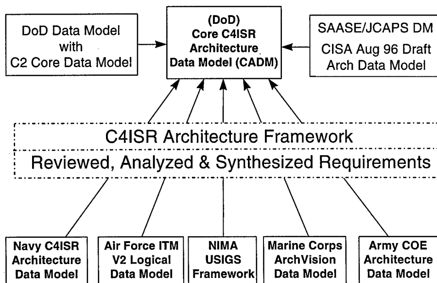
Figure 4-41. Sources for CADM Development
