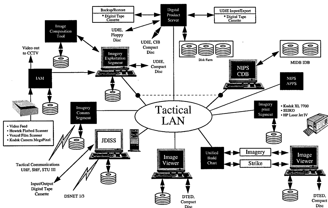
Figure 4-10b. System Interface Description, Intrasytem Perspective (SV-1) -- Notional Example
