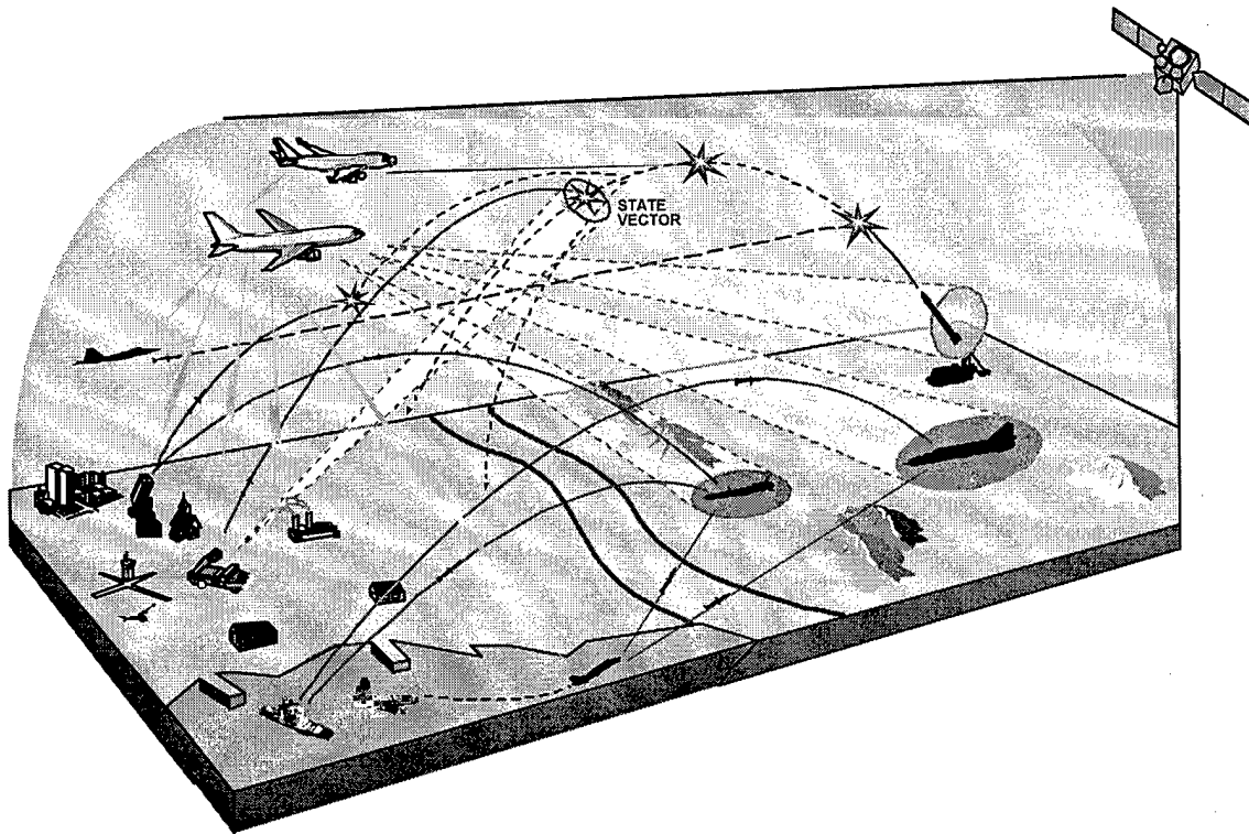
Figure 4-4b. High-level Operational Concept Graphic (OV-1) -- Theater Air Defense Example
