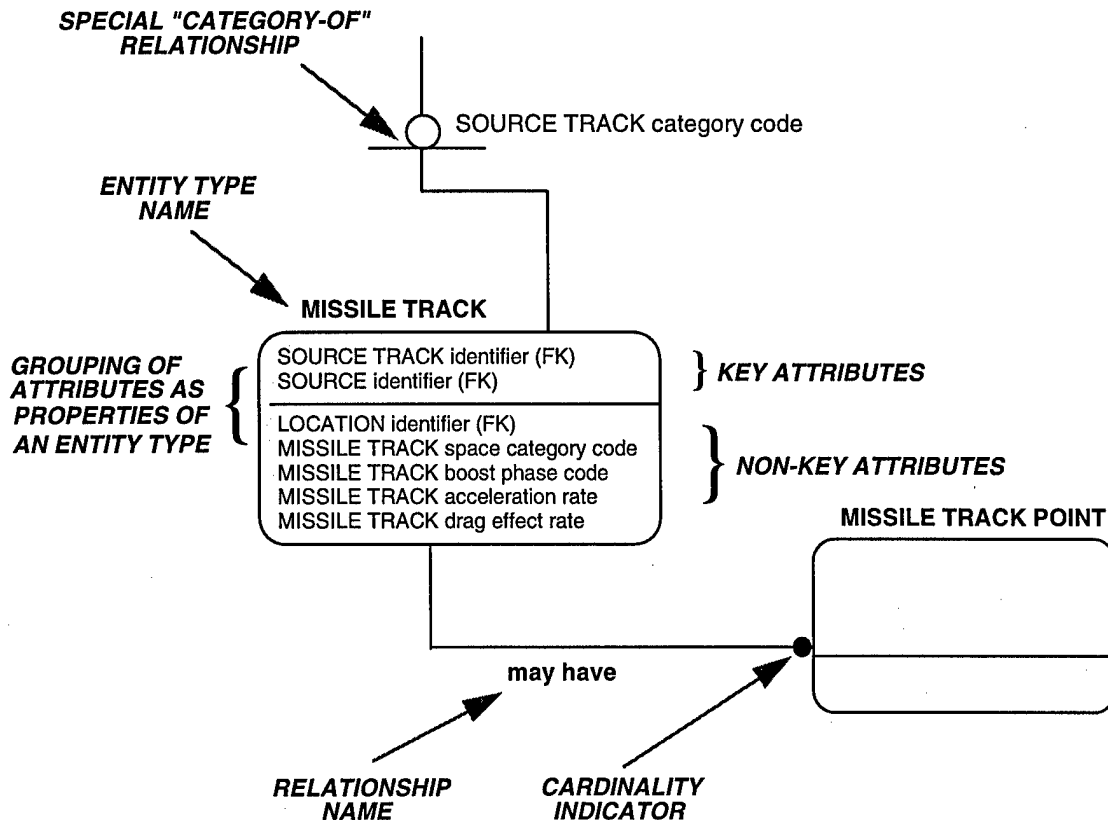
Figure 4-18b. Operational Rules Model (OV-6a) -- BMD Active Defense Example Illustrating the Legend for the Logical Data Model
