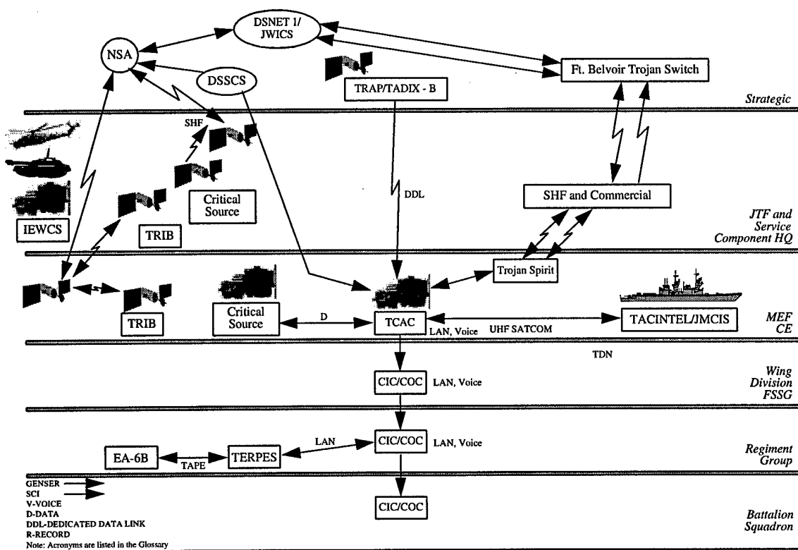
Figure 4-8d. System Interface Description, Internodal Perspective (SV-1) -- USACOM CIAD Example with Nodes Depicted By Echelon
