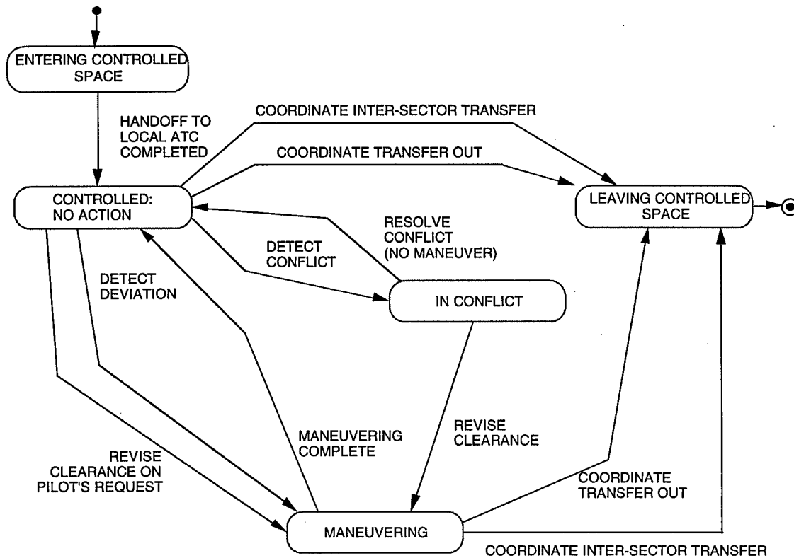
Figure 4-21. Operational State Transition Description (OV-6b) -- Air Traffic Operations Example
