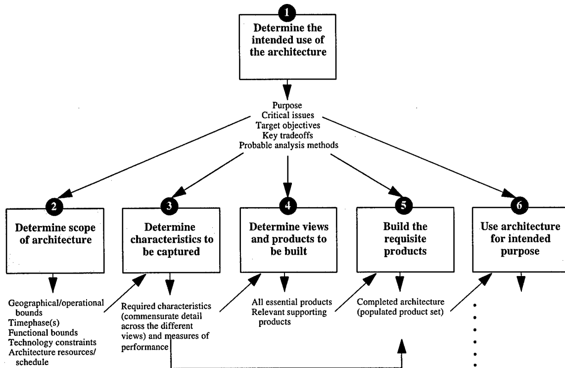
Figure 3-1. The Six-Step Process of Building an Architecture
