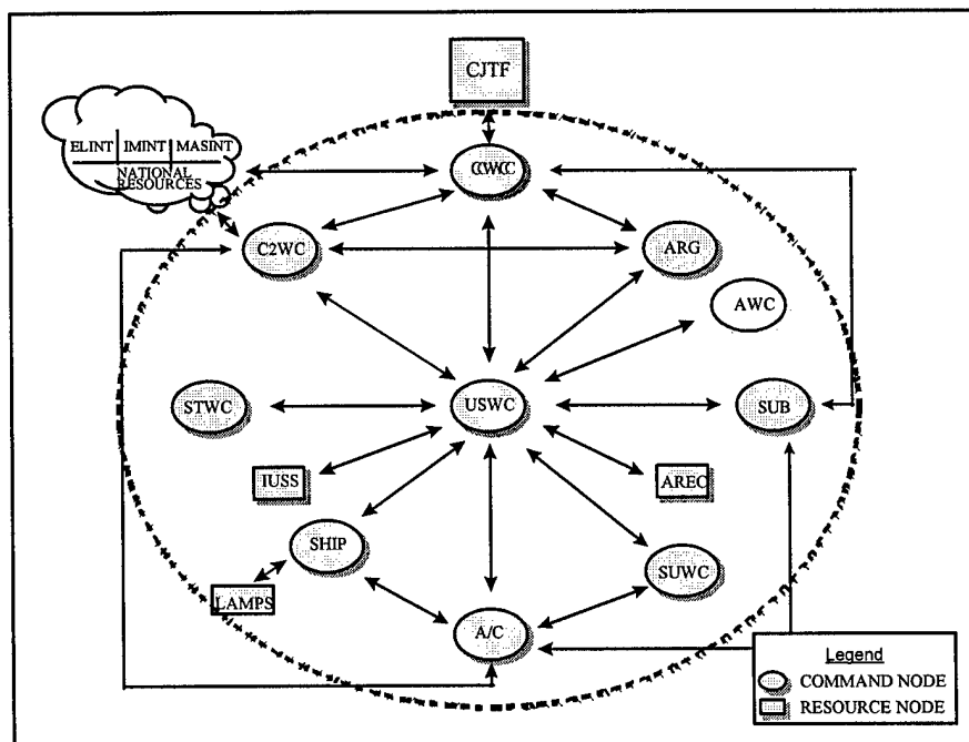
Figure 4-6f. Operational Node Connectivity Description (OV-2) -- Example Showing Multiple Node Types
