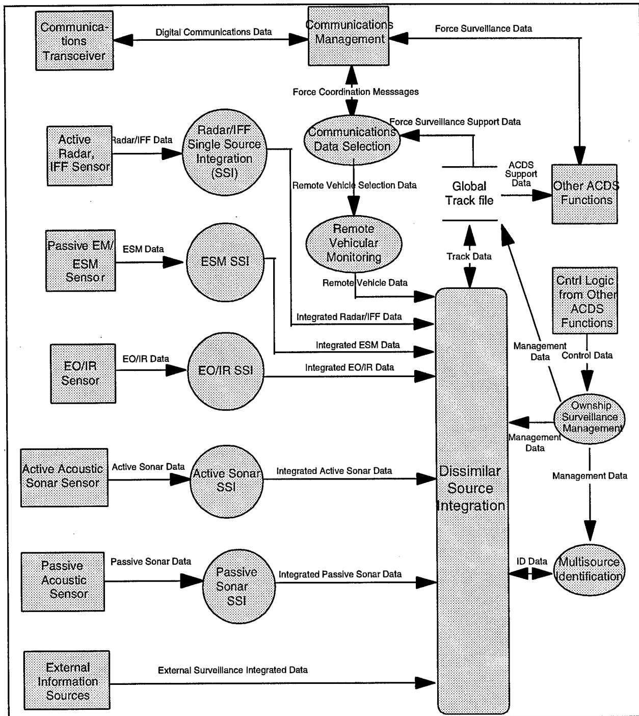
Figure 4-28. Systems Functionality Description (SV-4) -- Naval Sensor Functional Flow Diagram Example
