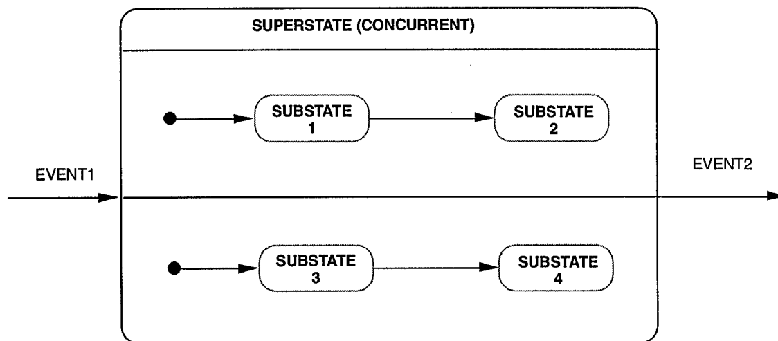
Figure 4-35b. System State Transition Description (SV-10b) -- Concurrent Activity State Structure Template
