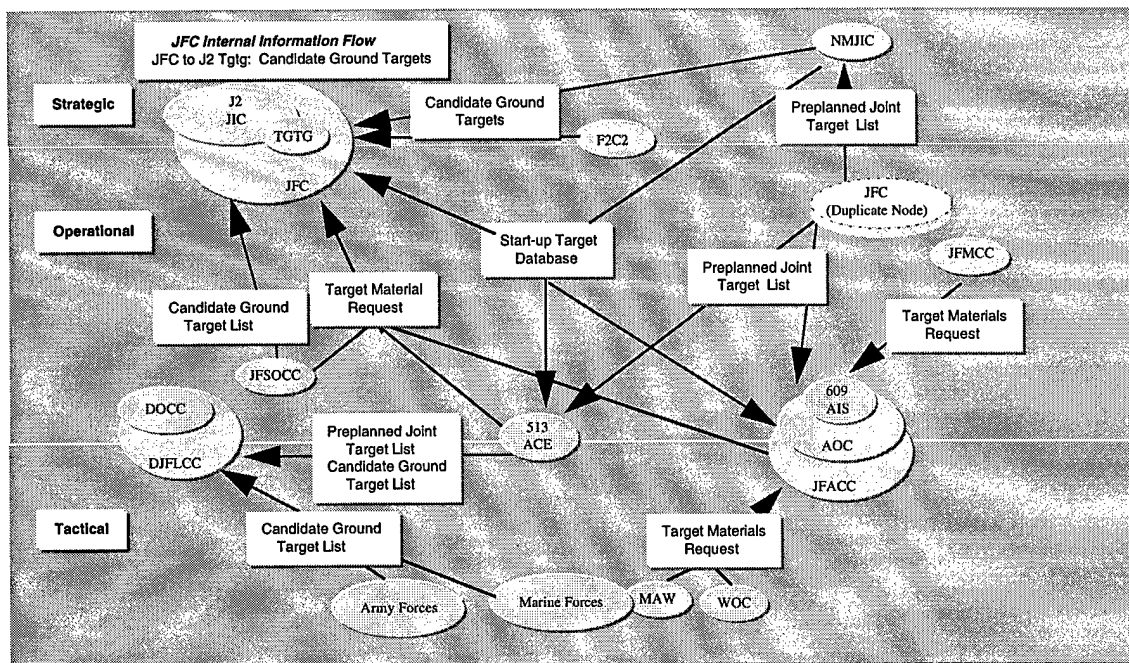
Figure 4-6d. Operational Node Connectivity Description (OV-2) -- Target Selection Example
