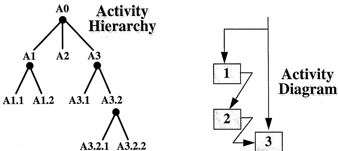
Figure 4-14. Activity Hierarchy Chart and Activity Diagram (OV-5) -- Templates
