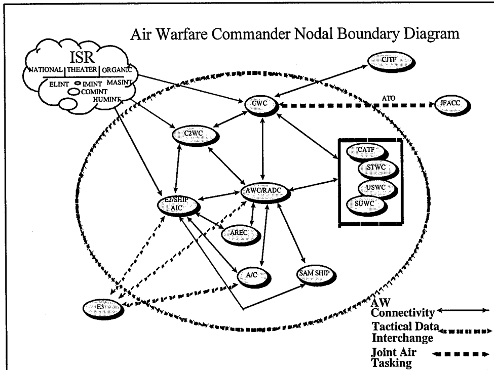
Figure 4-6e. Operational Node Connectivity Description (OV-2) -- Air Warfare Commander Example
