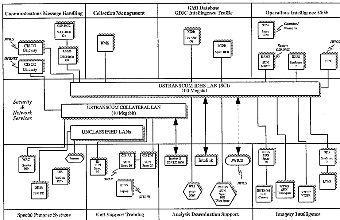
Figure 4-25d. Systems Communications Description, Intranodal Perspective (SV-2) -- TRANSCOM CIAD Example
