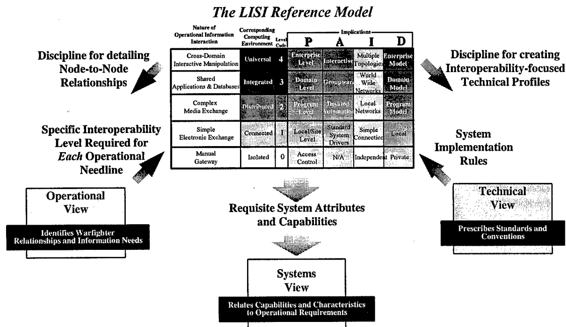
Figure D-4 LISI Relationship to Architecture Views
