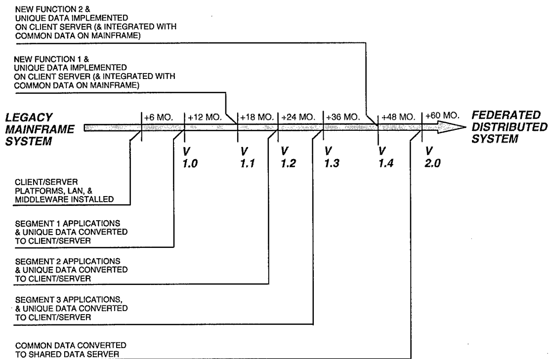
Figure 4-32b. System Evolution Diagram (SV-8) -- Evolution Example
