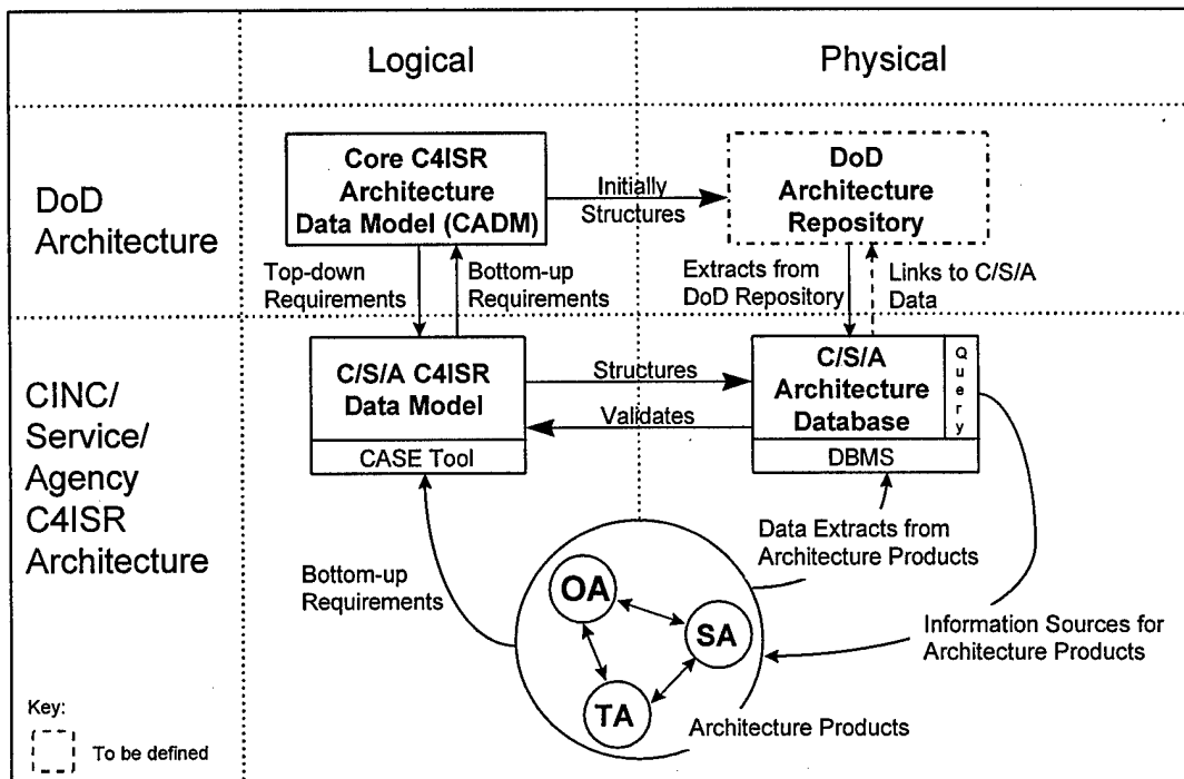
Figure 4-43. Potential Uses of the CADM
