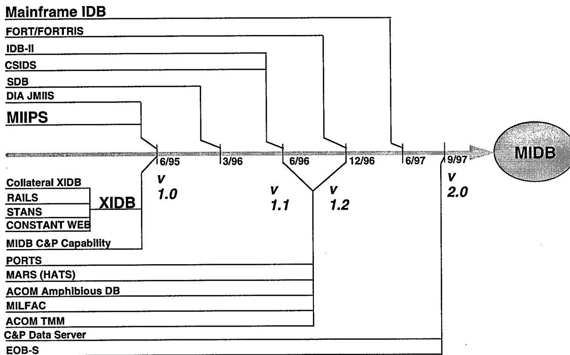
Figure 4-32a. System Evolution Diagram (SV-8) -- Migration Example
