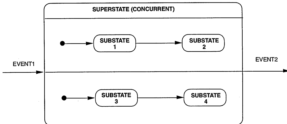
Figure 4-20b. Operational State Transition Description (OV-6b) -- Concurrent Activity State Structure Template
