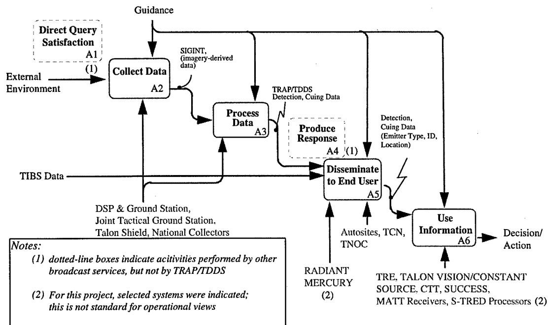
Figure 4-17. Activity Model (OV-5) -- UHF Intelligence Broadcast Service Example (with Overlays)
