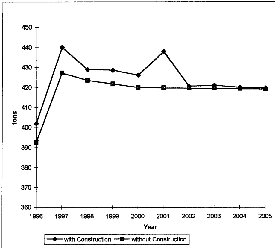
Figure D.5: AFB VOC Emission Comparisons
