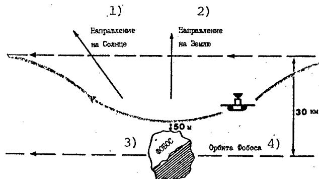
Fig. 3. Diagram of flight of "Fobos" space vehicle over surface. Relative flight velocity 2-5 m/s; flight time at altitude 50 m -- 15-20 minutes.
