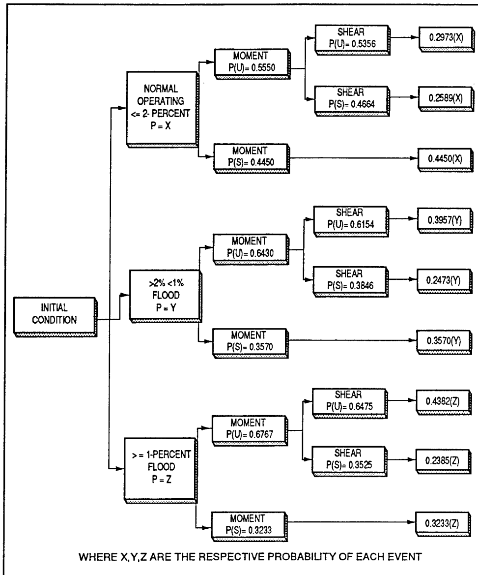
Figure 12. Event Tree for joint probabilities from the Monte Carlo Simulation
