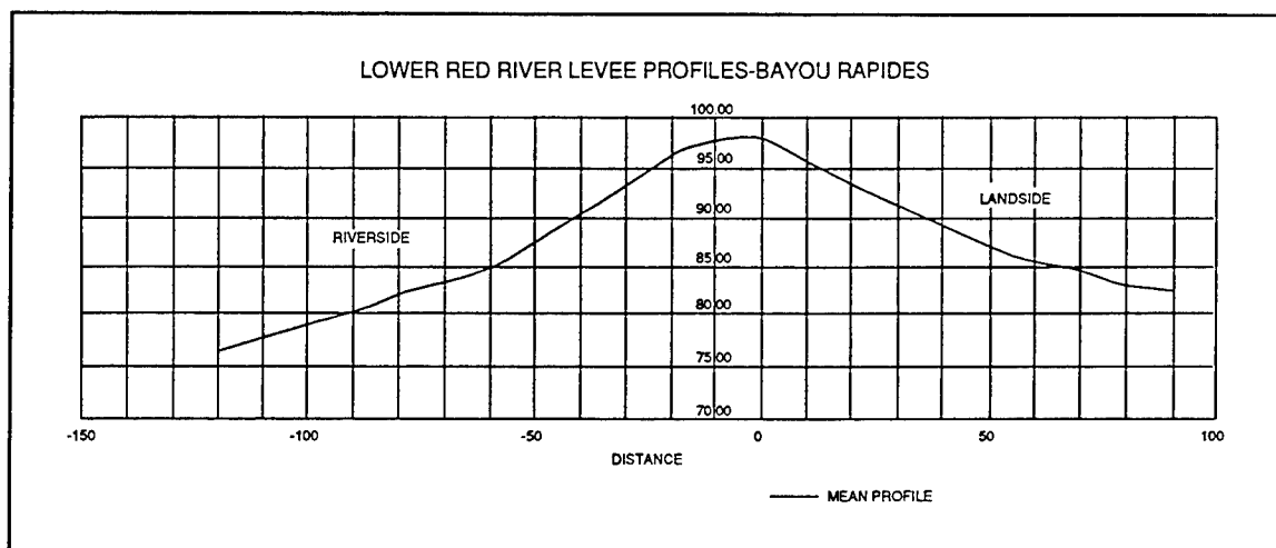
Figure 5. Mean profile of river levee
