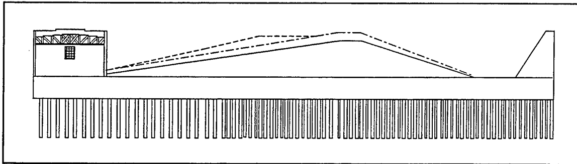
Figure 1. Cross section of drainage structure and pumping plant
