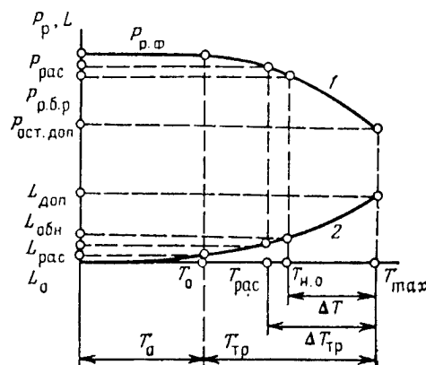
Figure 2. Determined Diagram of Ensuring Survivability Using Principle of Permissible Damage (Slow Growth of Cracks): 1--residual strength; 2--growth of cracks; loads: P_p --breaking; P_{pac} --calculated; P_{p.6.p} --breaking during safe flying life; P_{ост.дон} --minimum permissible. Length of crack: L_{дон} --maximum permissible; L_{обн} --minimum detectable; L_{pac} --corresponding to P_{pac} ; L_0 --initial length of crack at which P < P_p . Flying life: T_0 --before appearance of crack; T_{max} --maximum permissible; T_{tp} --period of growth of crack; T_{pac} --mean cycles between failure at which design tolerates P_{pac} ; \Delta T_{tp} --mean cycles between failure at which load-carrying capacity varies from P_{p.6.p} to P_{ост.дон}
