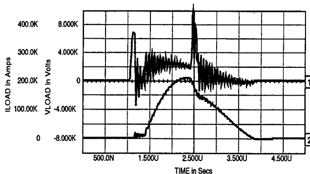
SPICE Simulation of DPF Load Response with solid-state driver charged to 7 kV - Trace 1: V load : 2 kV/div - Trace 2: I load : 50 kA/div - Horizontal: 0.5 μsec/div
