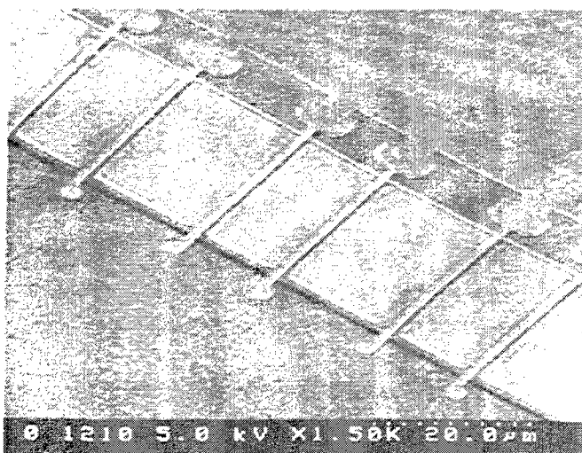
Figure 9 (a and b): T-Gate Fabrication Based on a Bilayer Resist Process, Resulting in a Free Standing "T" Structure. A device cell made up of six gates is also shown.
