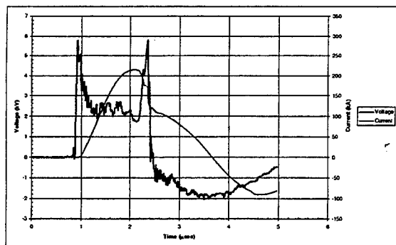
Measured DPF Response 29 μF charged to 7 kV
