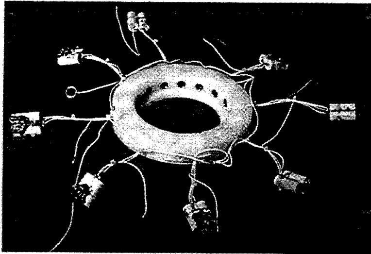
Figure 19: Hollow Cathode Array with Pulse Discharge Capacitors
