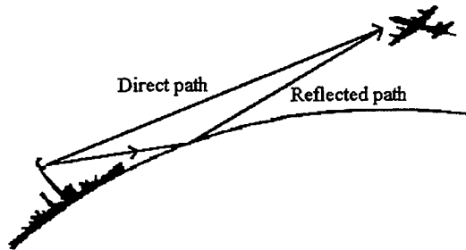
Figure 3-7: Surface reflection.
