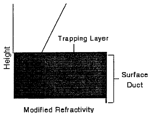
Figure 3-3: Surface duct.
