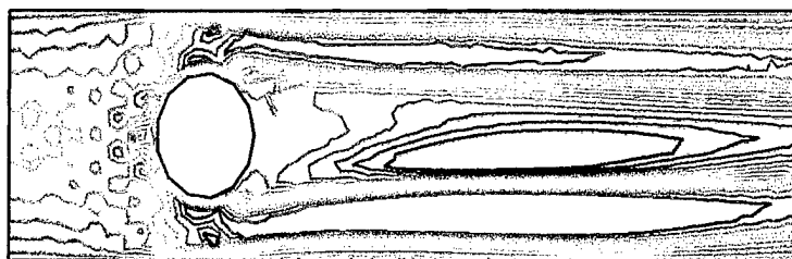
b) u Velocity Sensitivity Contours, Projected Derivatives: L = 6
