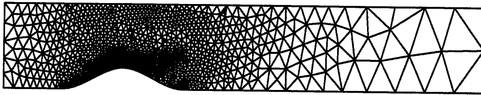
c) Fourth Adapted Mesh (3962 Nodes/1901 Elements)
