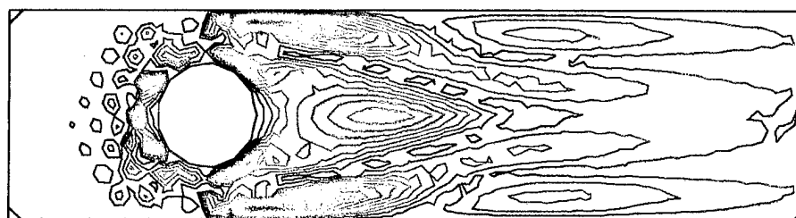
a) Error in u Sensitivities - Unprojected Derivatives
