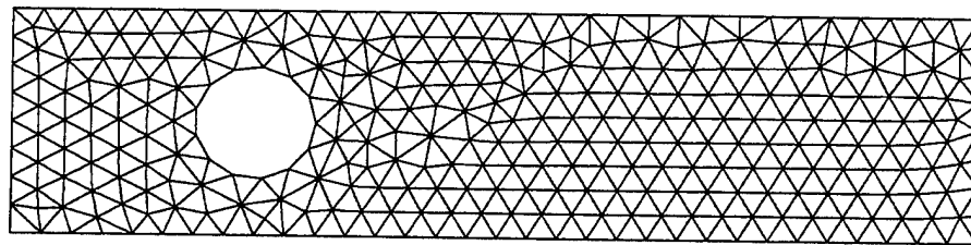
a) Initial Mesh (1219 nodes/563 elements)
