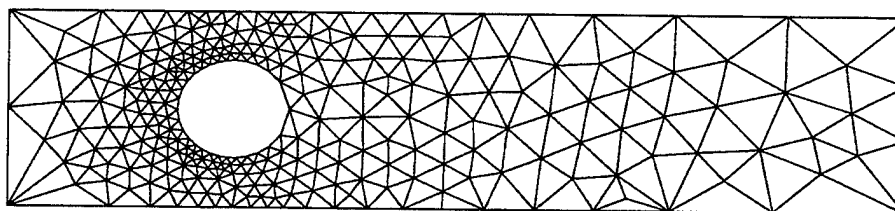
d) First Adapted Mesh - Flow & Projected Sens (1066 nodes/496 elements)
