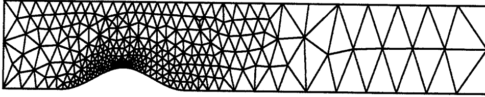
b) Second Adapted Mesh (1094 Nodes/505 Elements)
