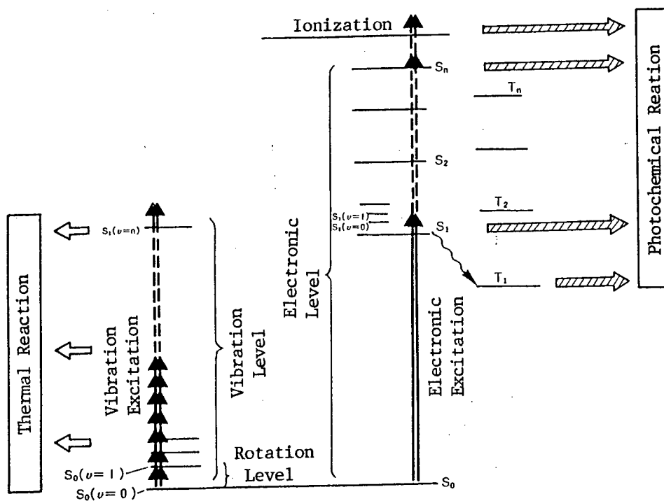
Figure 1. Lasers and Relevant Chemical Reactions (Vibration Excitation and Electronic Excitation)
