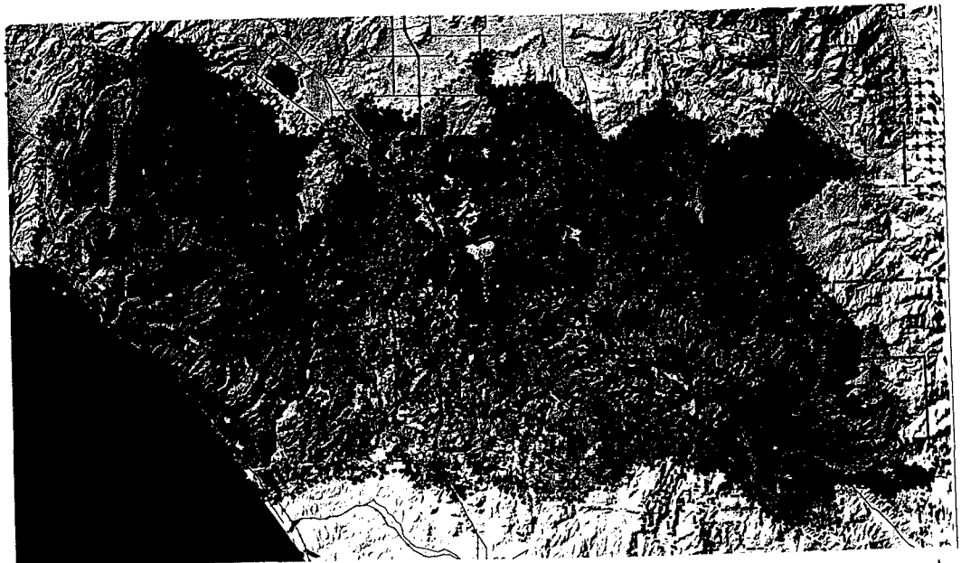
Species Richness: 1990+
