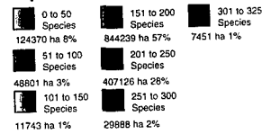
Species Richness: 1990+
