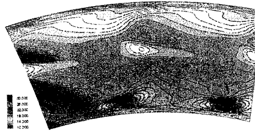
(c) TRACE-S using extended k-\epsilon model (Lisiewicz)
