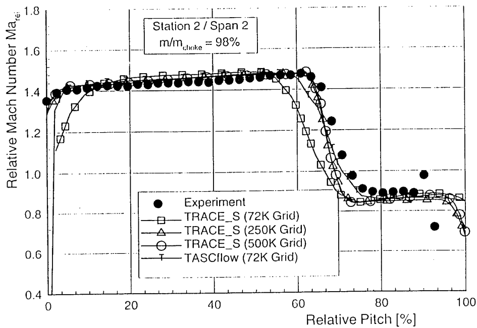
Fig 3.14 Mach number variation across the pitch at mid-span (Hildebrandt)
