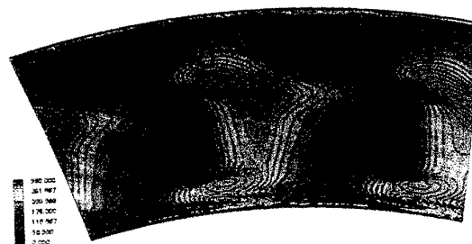
(b) TRACE-S using extended k-\epsilon model (Lisiewicz)
