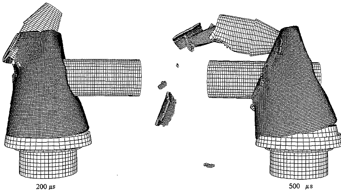
Figure 3. DYN3D Simulation Results Showing Deformed Fuze and Ogive Fragmentation at 200 and 500 \mu s.
