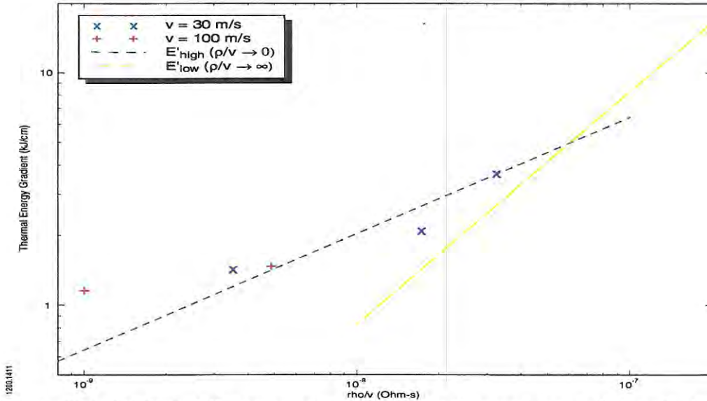
Figure 8. Calculated 3-D component of the thermal energy per unit length in rail plus cladding for 30 and 100 m/s armature velocities. The curve E'_{low} is the theoretical prediction for large \rho/v . The curve E'_{high} has the predicted \left(\frac{\rho}{v}\right)^{1/2} dependence for small \rho/v with a coefficient adjusted to give the best fit to the calculated points.
