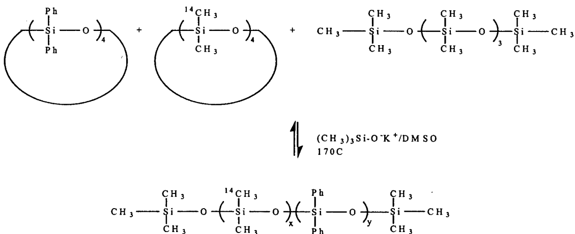
Figure 10. Synthesis of ^{14}\text{C} -labeled Polydiphenyldimethylsiloxane
