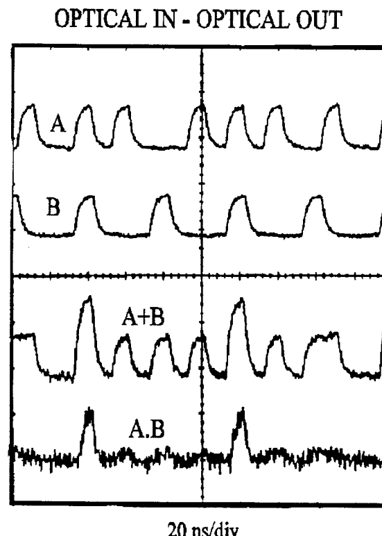
(c) OPTICAL LOGIC INPUTS OPTICAL LOGIC OUTPUT
