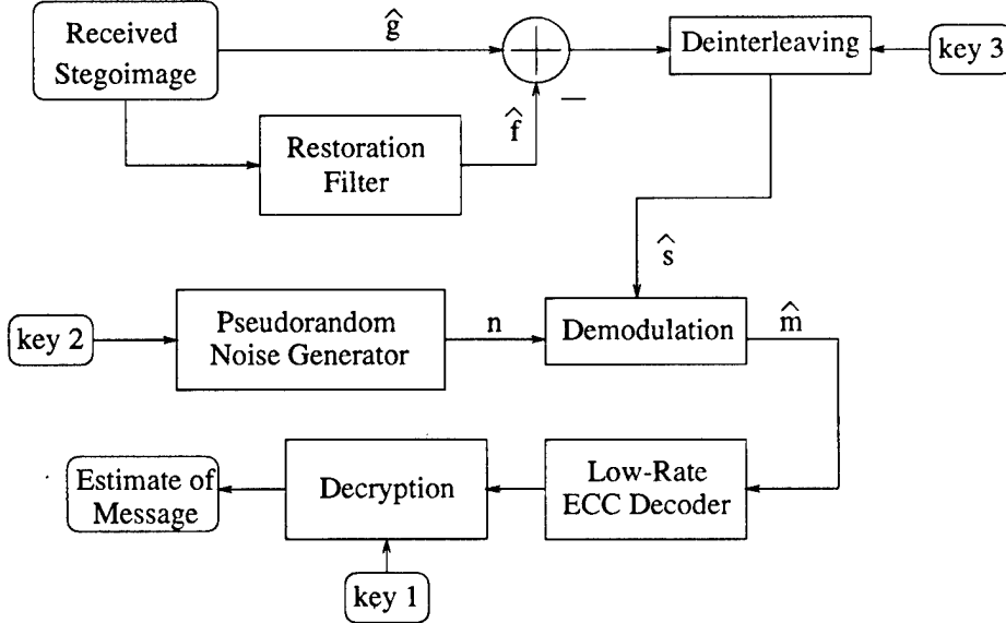
Figure 3. SSIS Decoder.
