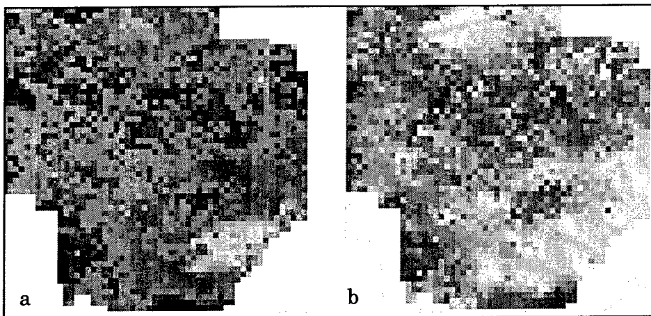
Figure 10. The average percent aerial cover of vegetation (a) and average index of habitat suitability (b) for desert tortoises after running scenario 3a for 250 years for Fort Irwin. The average was obtained from 100 simulations of scenario 3a. Figures 5a and 6b show the average percent aerial cover of vegetation and index of habitat suitability, respectively, at time 0 for scenario 3a. No new training occurred in the model after time step 0. Darker shades represent higher densities of vegetative cover (a) and habitat better suited for tortoises (b).
