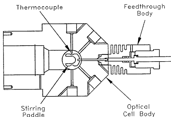
Figure 6. Cross-section of the stirred optical cell showing the stirring mechanism.
