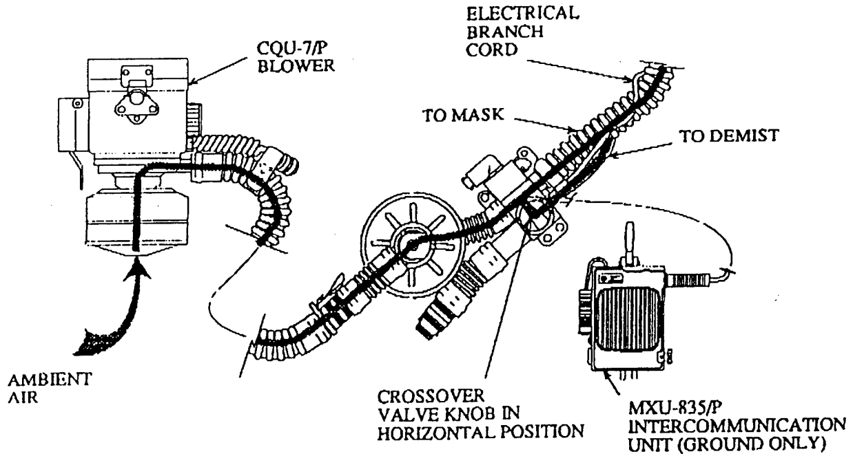
MBU-19/P GROUND OR NON-OXYGEN FLIGHT OPERATING MODE.
