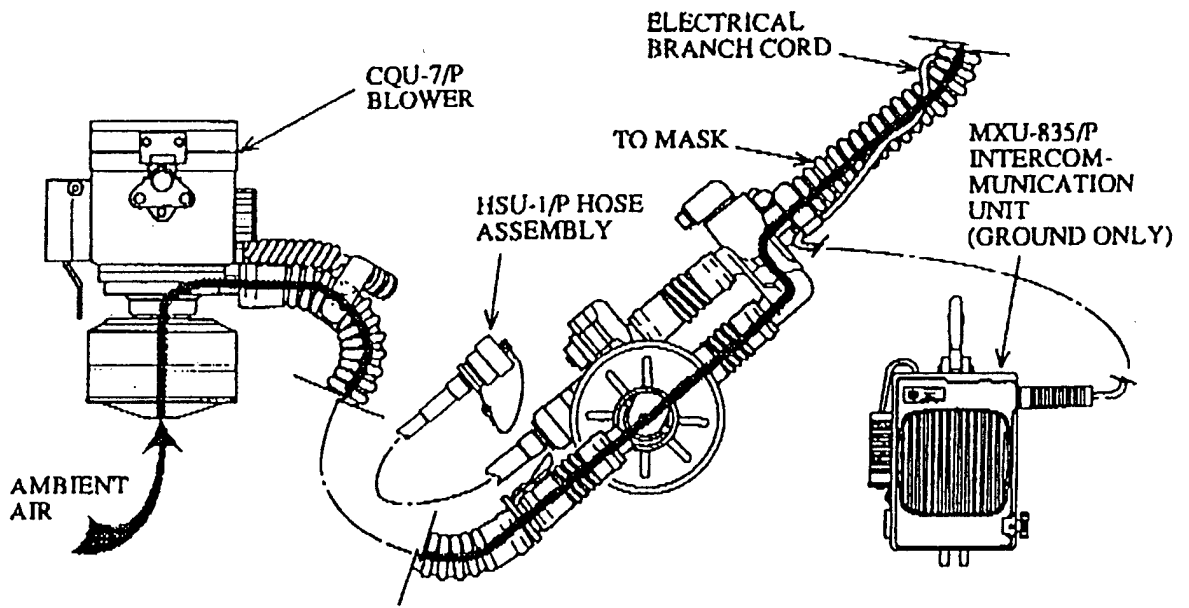
MBU-18/P GROUND OPERATING MODE.
