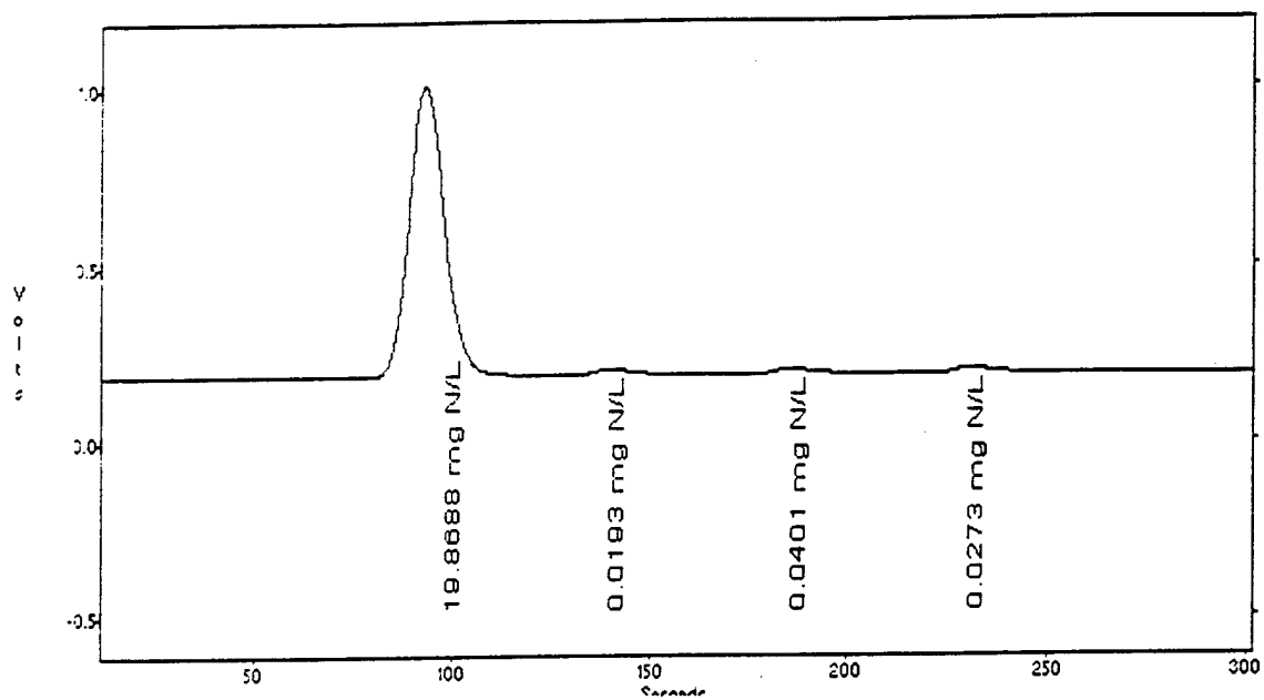
Figure 4. Carryover
