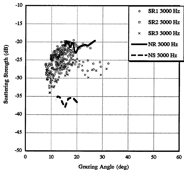
Fig. 7 — Bottom backscattering strength as a function of grazing angle at 3000 Hz for LWAD SCV 97 scattering sites
