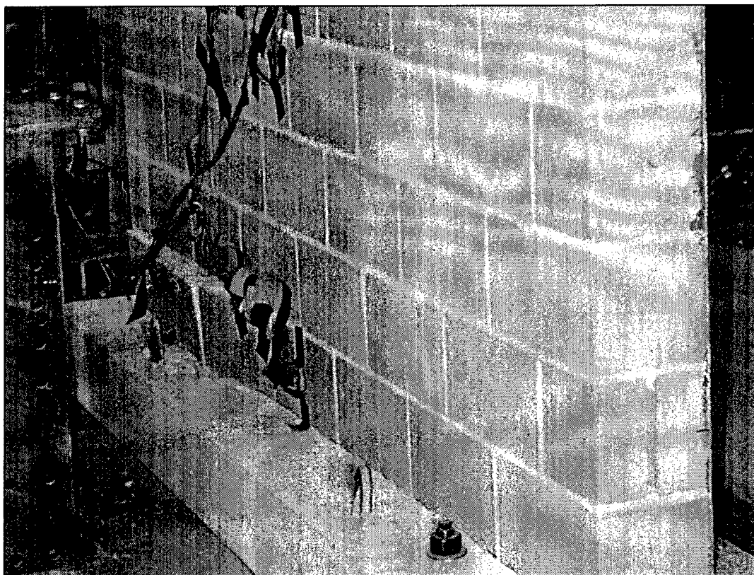
Figure A15. Out-of-plane facial slippage of bottom course CMU, inside of the north wall.
