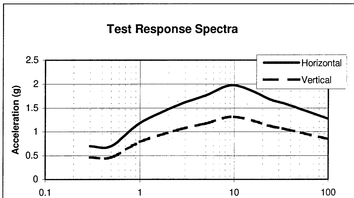
Figure 4. Horizontal and vertical ground spectra, 5% damping.
