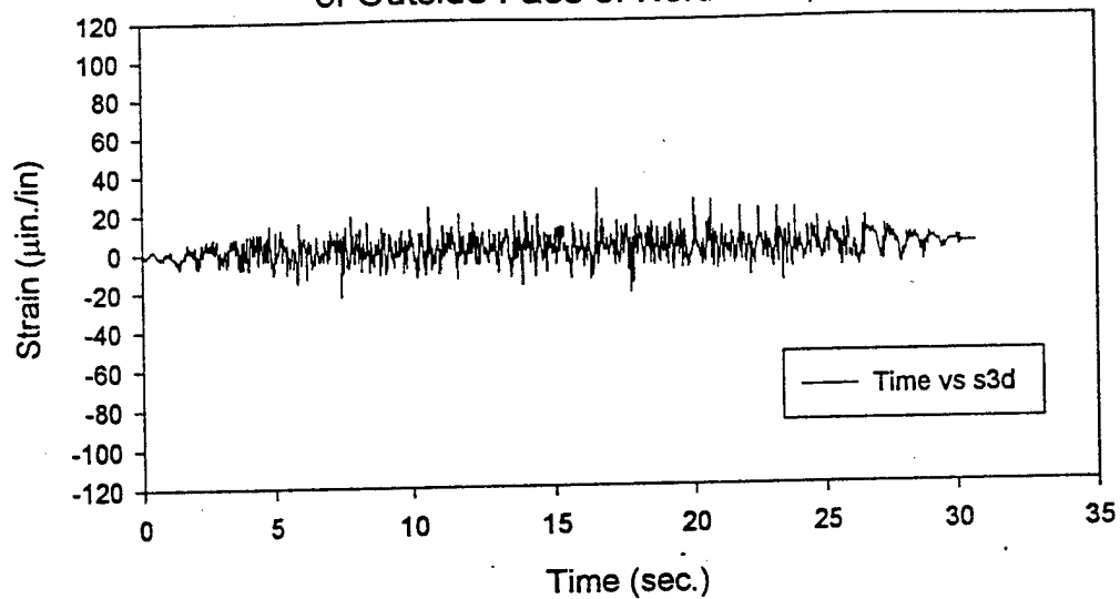
Horizontal Strain at Center of Outside Face of North Wall, EQ-6
