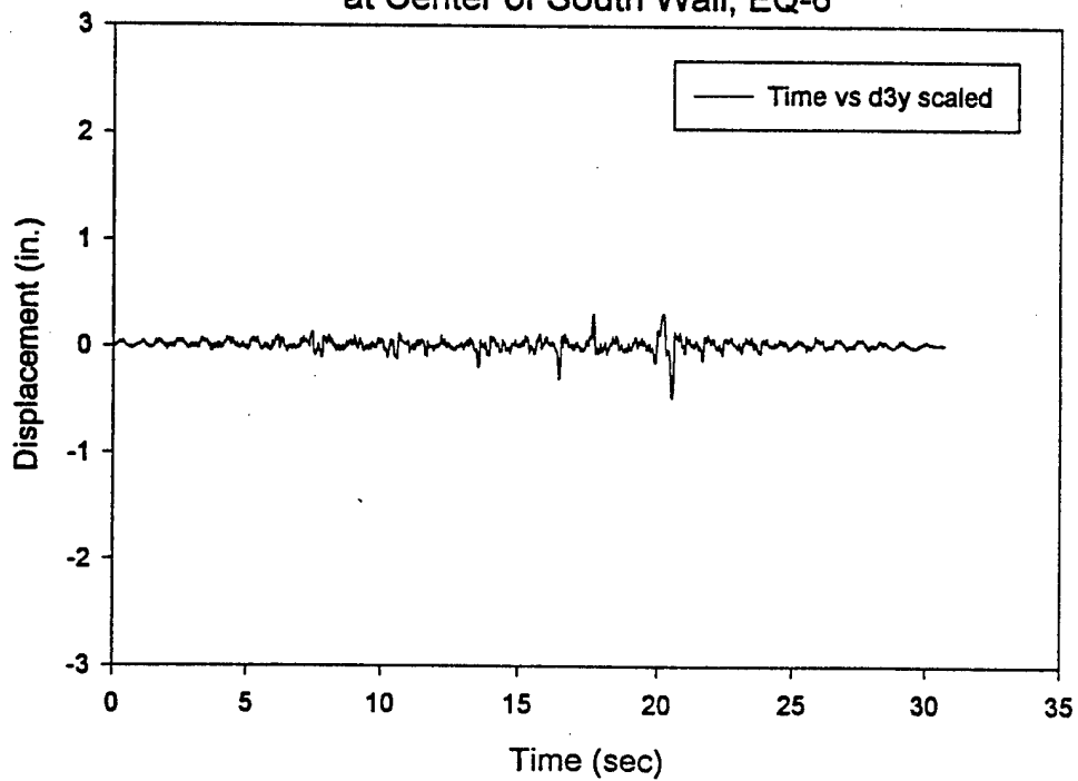
In-Plane Displacement at Center of South Wall, EQ-6
