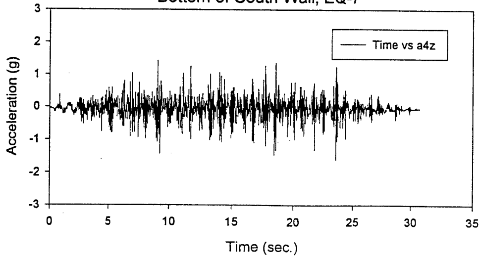
Vertical Acceleration at Bottom of South Wall, EQ-7
