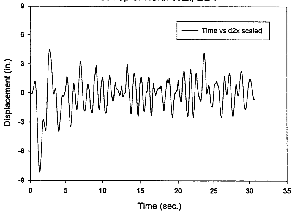
Out-of-Plane Displacement at Top of North Wall, EQ-7
