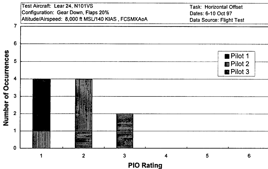
Figure D20 Horizontal Offset Landing PIO Ratings - MXAOA
