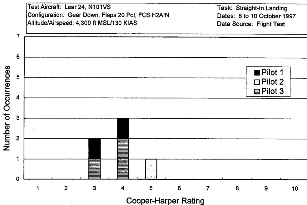
Figure D13 Straight-In Landing Cooper-Harper Ratings - H2AIN
