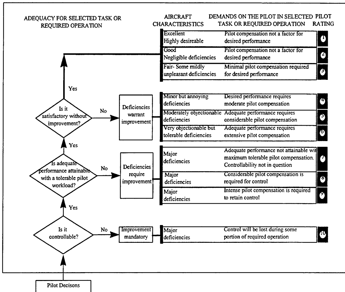
Figure B4 Cooper-Harper Rating Scale
