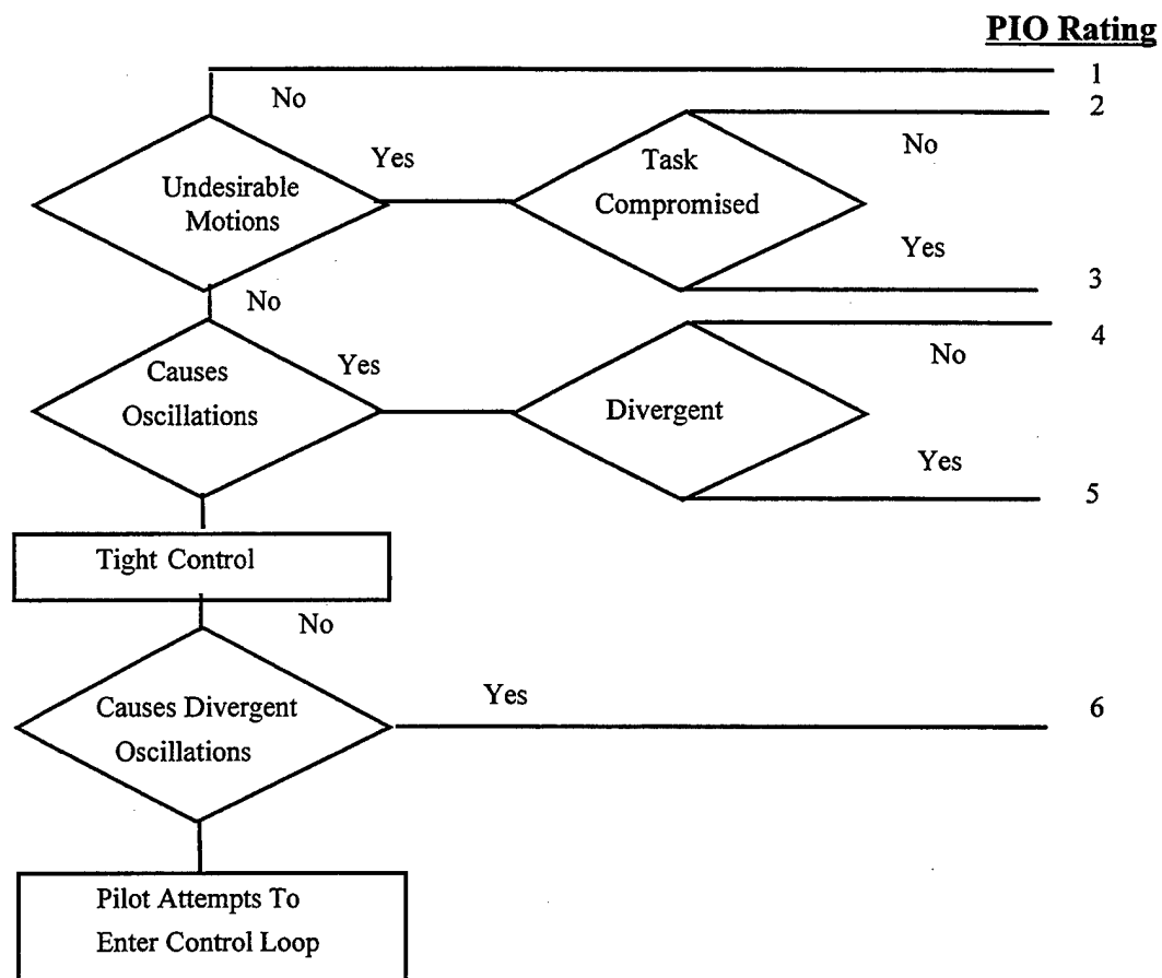
Figure B5 Pilot-in-the-Loop Oscillation Rating Decision Tree
