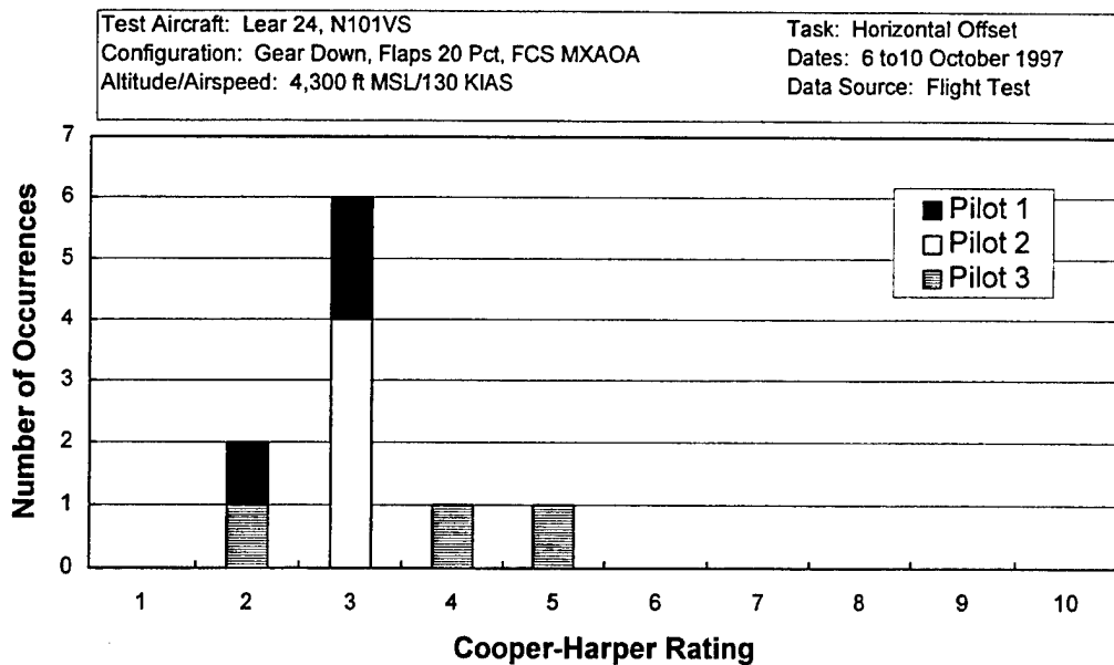
Figure D19 Horizontal Offset Landing Cooper-Harper Ratings - MXAOA
