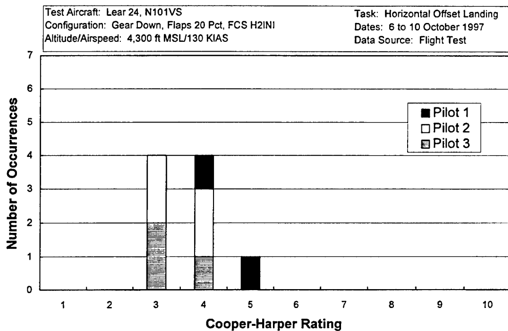
Figure D11 Horizontal Offset Landing Cooper-Harper Ratings - H2INI
