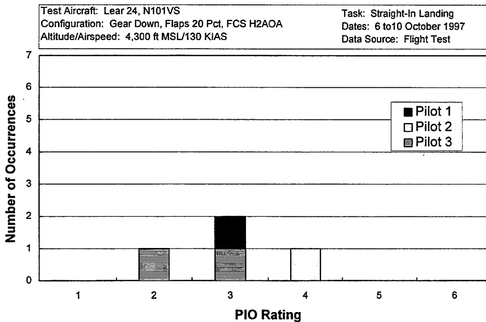
Figure D6 Straight-In Landing PIO Ratings - H2AOA
