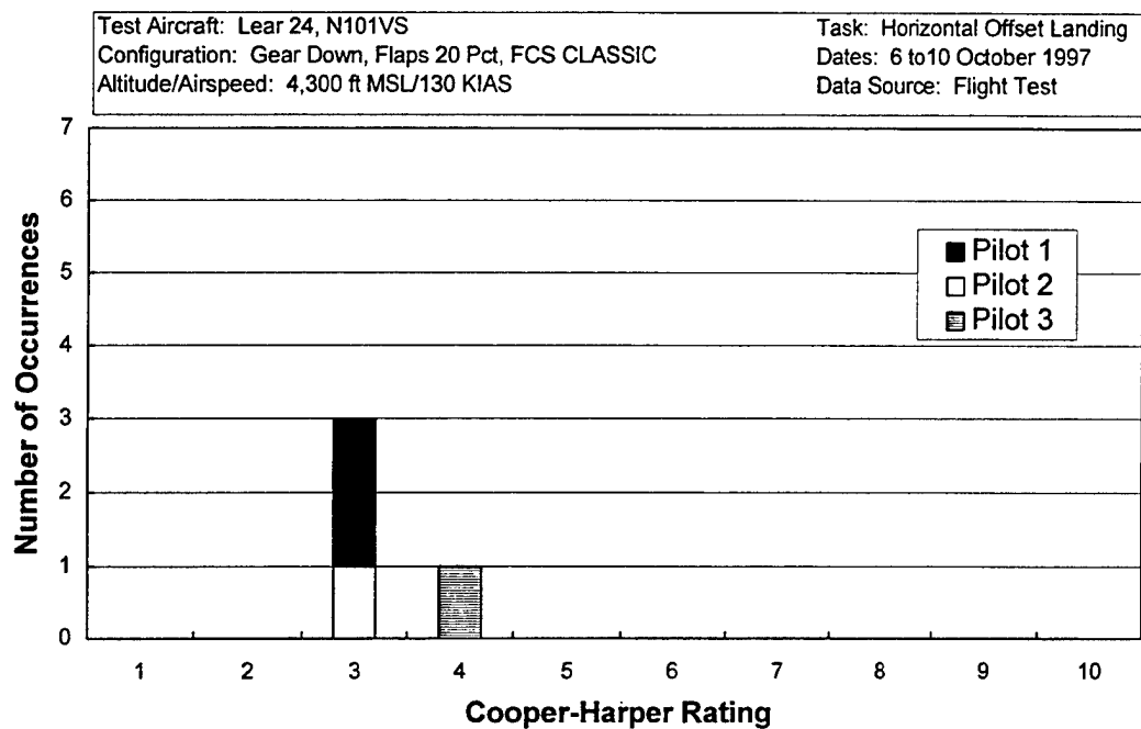
Figure D3 Horizontal Offset Landing Cooper-Harper Ratings - CLASSIC
