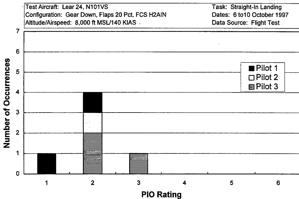
Figure D14 Straight-In Landing PIO Ratings - H2AIN
