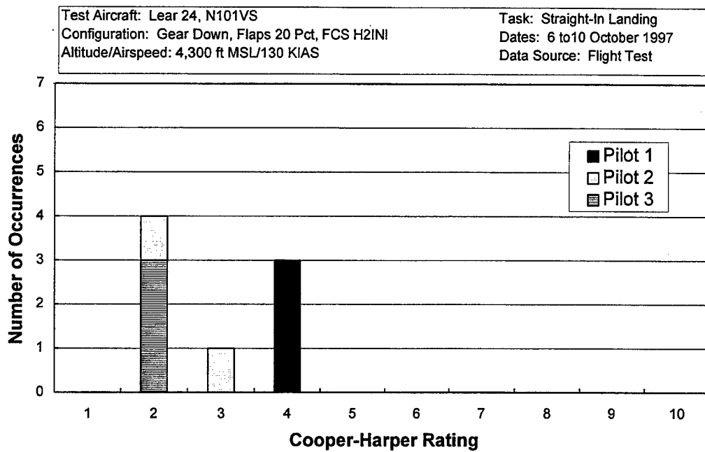
Figure D9 Straight-In Landing Cooper-Harper Ratings - H2INI
