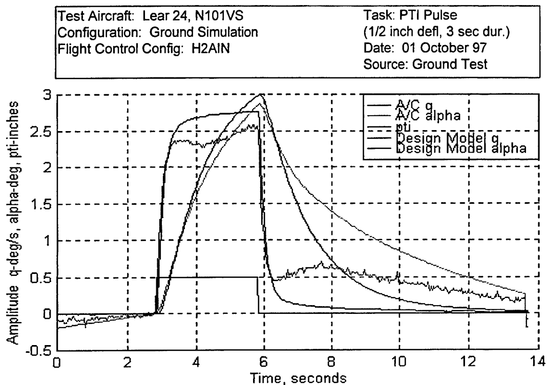
Figure C4 Ground Test Closed-Loop q and \alpha Time Responses - H2AIN
