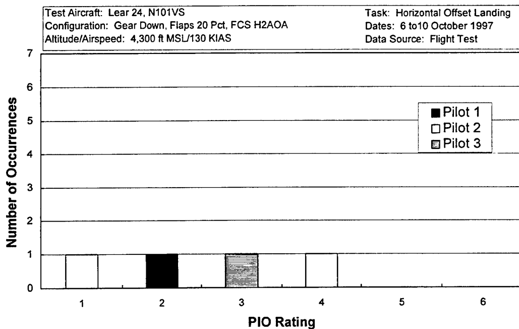
Figure D8 Horizontal Offset Landing PIO Ratings - H2AOA
