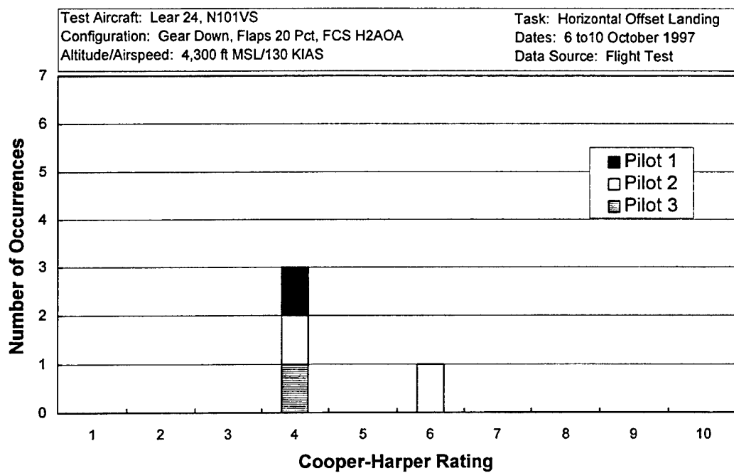
Figure D7 Horizontal Offset Landing Cooper-Harper Ratings - H2AOA
