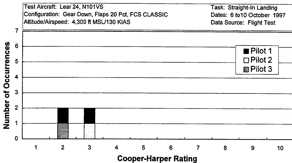
Figure D1 Straight-In Landing Cooper-Harper Ratings - CLASSIC
