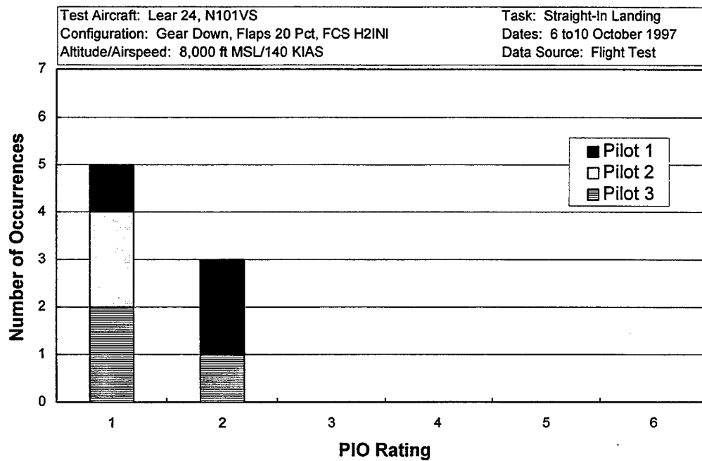
Figure D10 Straight-In Landing PIO Ratings - H2INI
