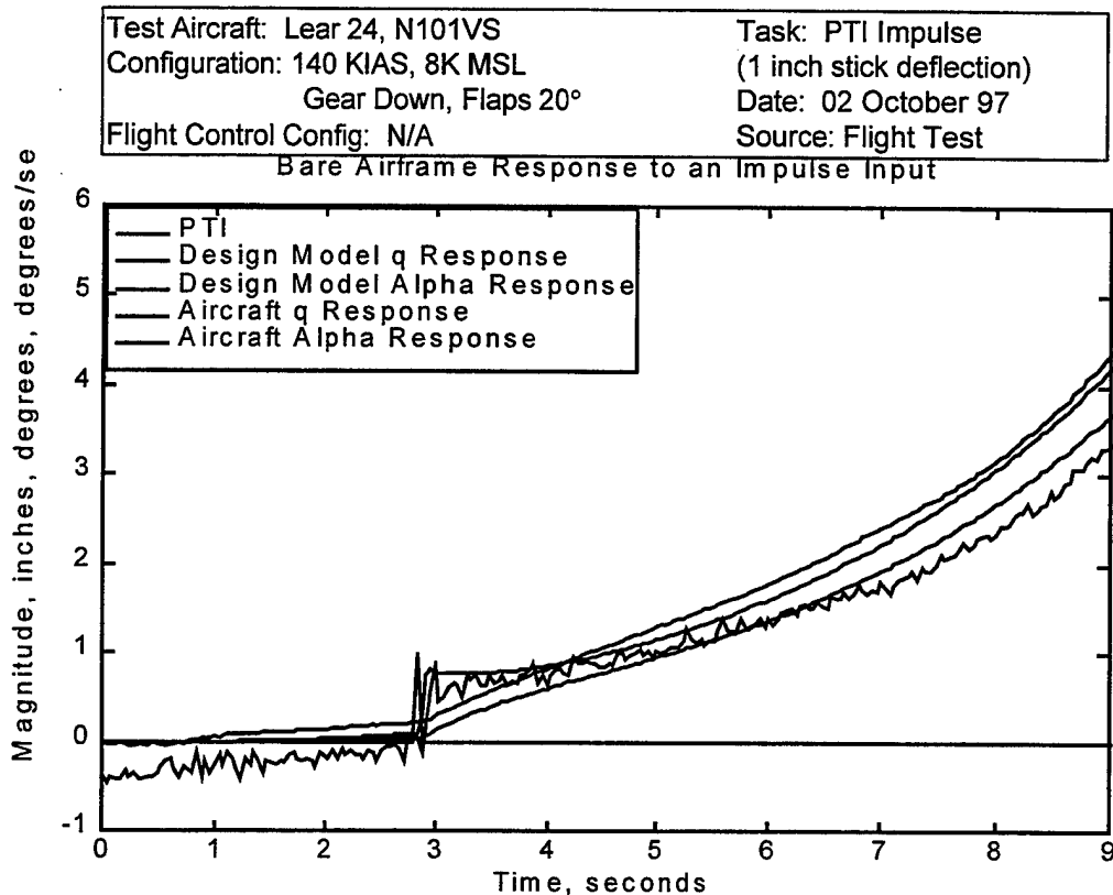
Figure C6 Bare Airframe Time Responses to an Impulse Input
