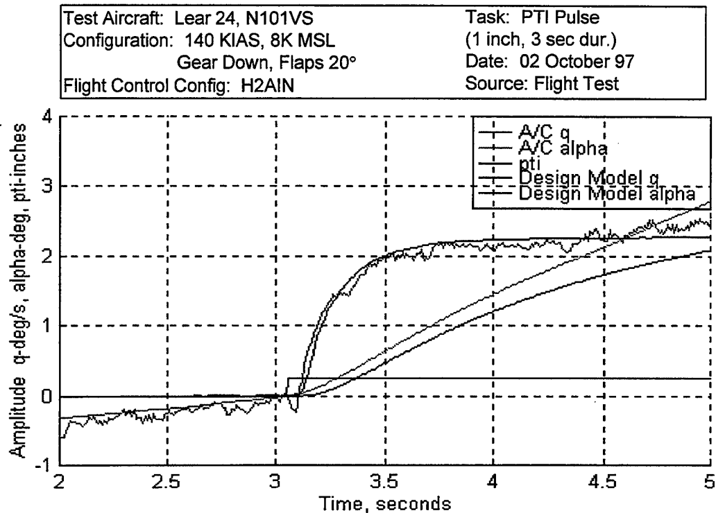
Figure C10 Flight Test Closed-Loop q and \alpha Time Responses - H2AIN
