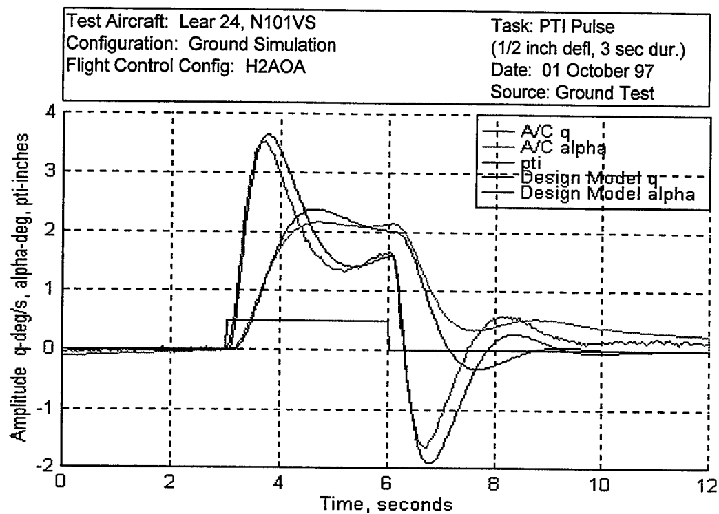
Figure C2 Ground Test Closed-Loop q and \alpha Time Responses - H2AOA
