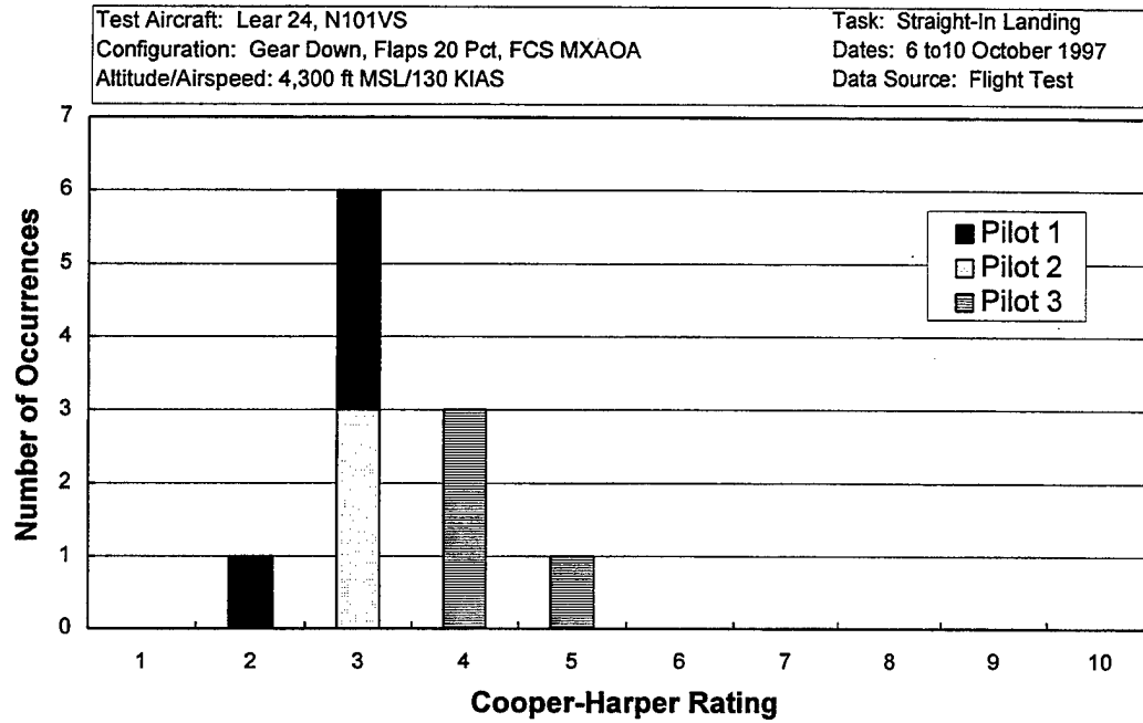
Figure D17 Straight-In Landing Cooper-Harper Ratings - MXAOA
