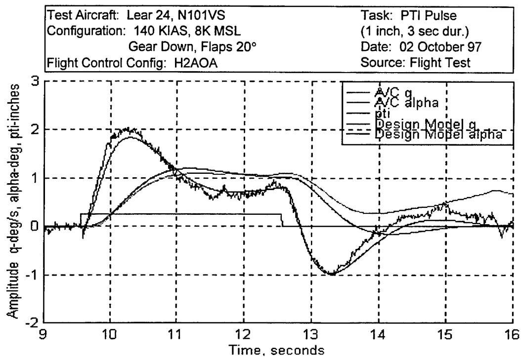
Figure C8 Flight Test Closed-Loop q and \alpha Time Responses - H2AOA
