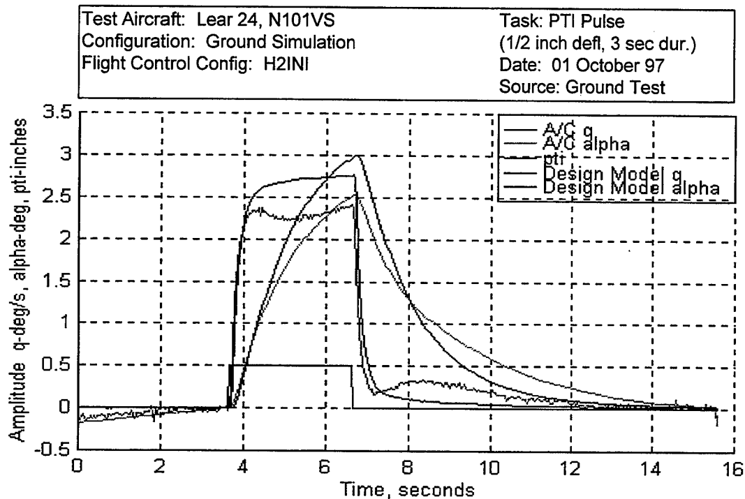
Figure C3 Ground Test Closed-Loop q and \alpha Time Responses - H2INI
