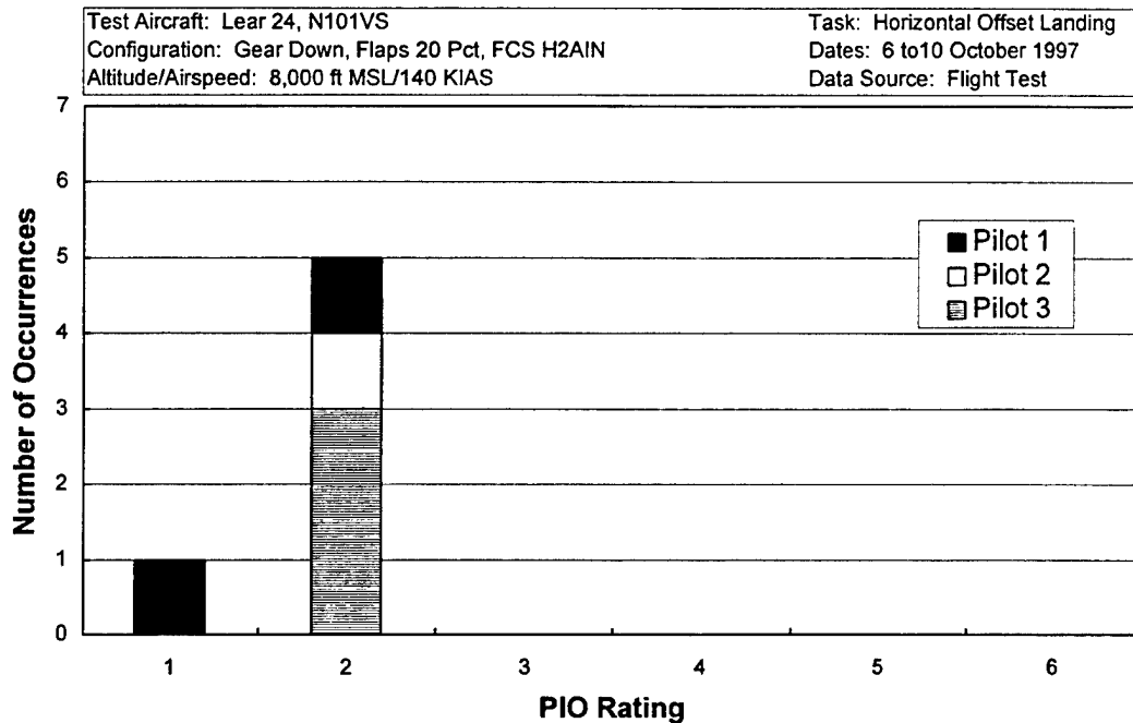
Figure D16 Horizontal Offset Landing PIO Ratings - H2AIN
