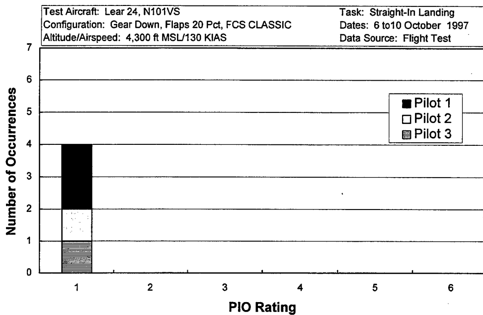
Figure D2 Straight-In Landing PIO Ratings - CLASSIC
