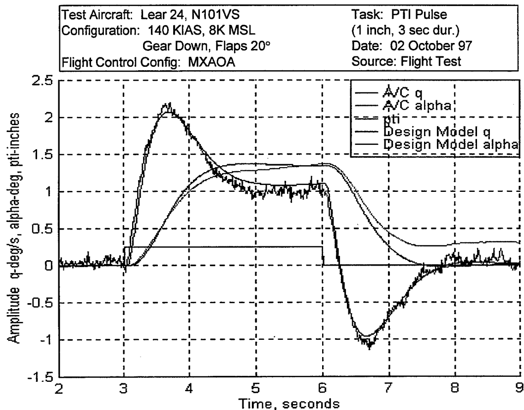
Figure C11 Flight Test Closed-Loop q and \alpha Time Responses - MXAOA
