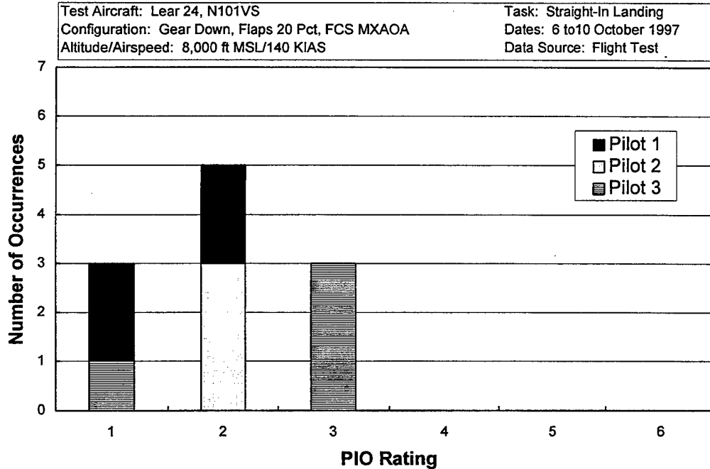
Figure D18 Straight-In Landing PIO Ratings - MXAOA
