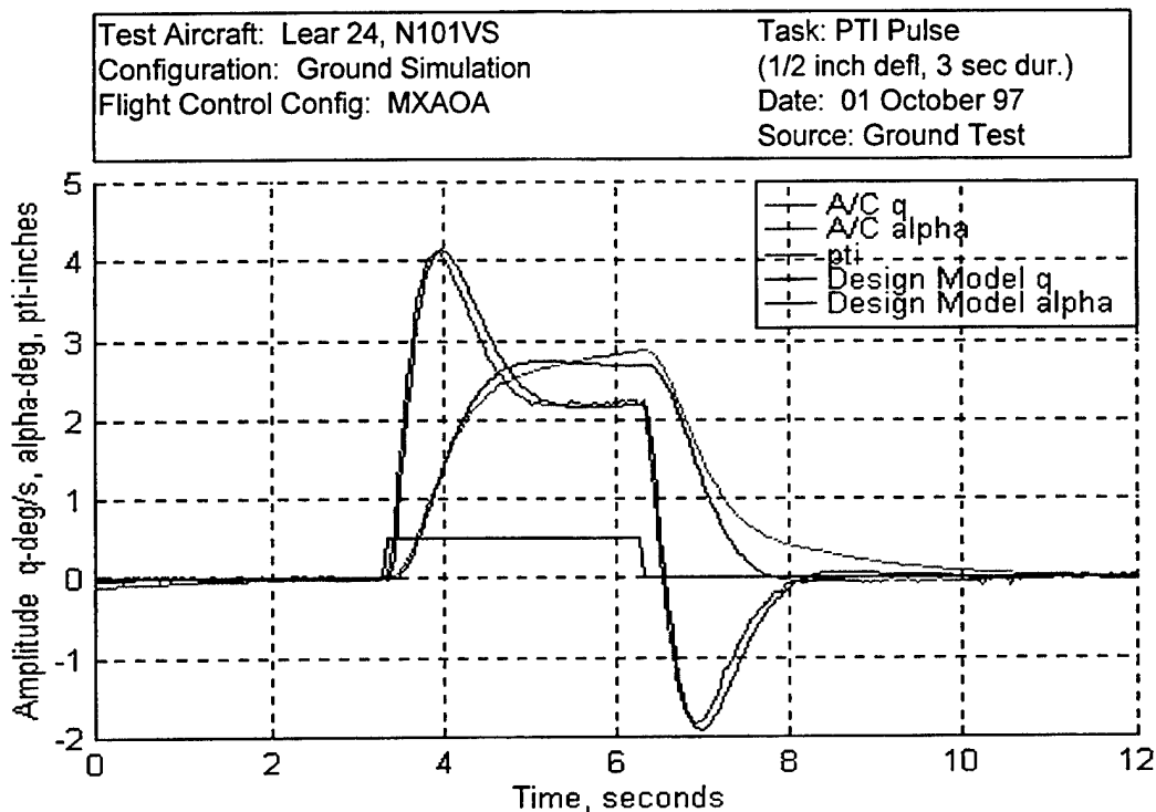
Figure C5 Ground Test Closed-Loop q and \alpha Time Responses - MXAOA
