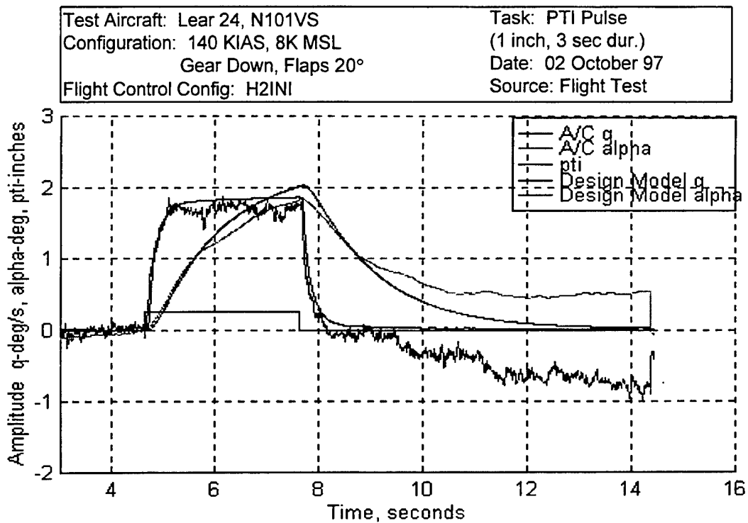
Figure C9 Flight Test Closed-Loop q and \alpha Time Responses - H2INI
