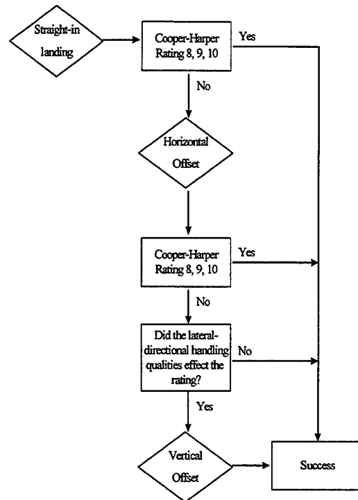
Figure 2 Landing Task Decision Tree
