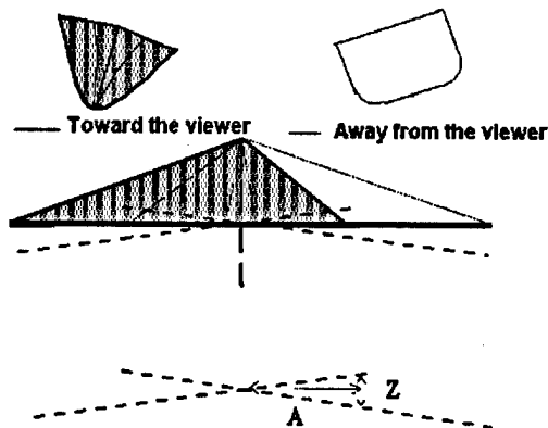
Figure 5. Profile view of two reciprocal lines run over a flat seafloor. The apparent across-track profiles (dashed lines) show a roll offset of 5 degrees. The depth difference Z and across-track distance A can be used to compute the roll offset. (Figure adapted from A. Godin.)
