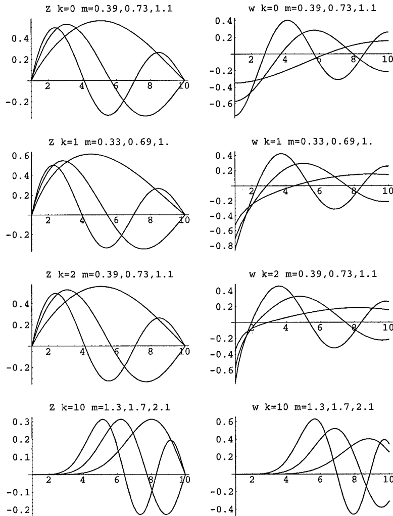
FIG. 5.1. Typical modes of \xi (left) and \omega (right) vs. radius.
