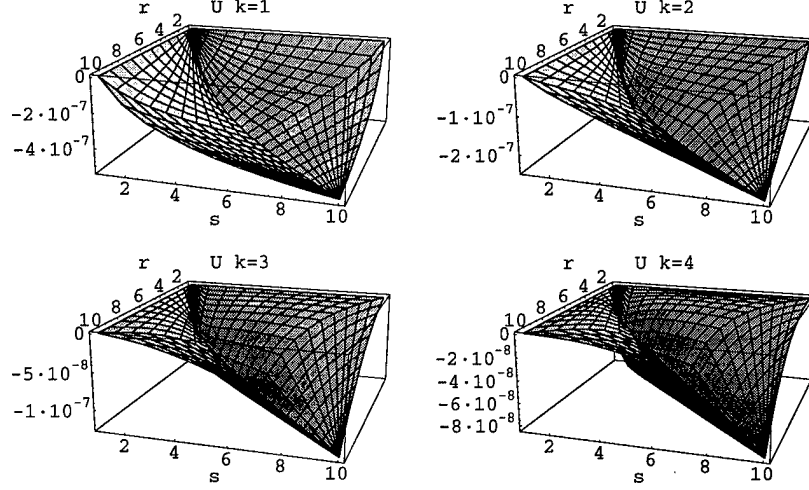
FIG. 7.1. Feedback at r due to disturbance in \xi_k at s for \epsilon = 0.001 and k = 1, \dots, 4 .
