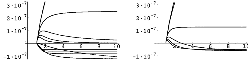
FIG. 7.3. Left: Boundary control (positive traces) and colocated control (negative traces) as functions of the radial location of the disturbance vortex for \epsilon = 0.001 and k = 0, \dots, 5 . Right: Sum of boundary control and colocated control. Within the region R \ll 1/\sqrt{\epsilon} , boundary control dominates for |k| \leq 2 or sufficiently close to the wall.
