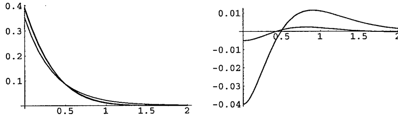
FIG. 6.2. Spatial form of the optimal feedback kernel for the heat equation on an infinite line. Left: the exact \kappa (6.11) and its rational approximations \kappa_1 and \kappa_2 as functions of s for \epsilon = 1 . Right: error in the two rational approximations shown using expanded vertical scale. See text.
