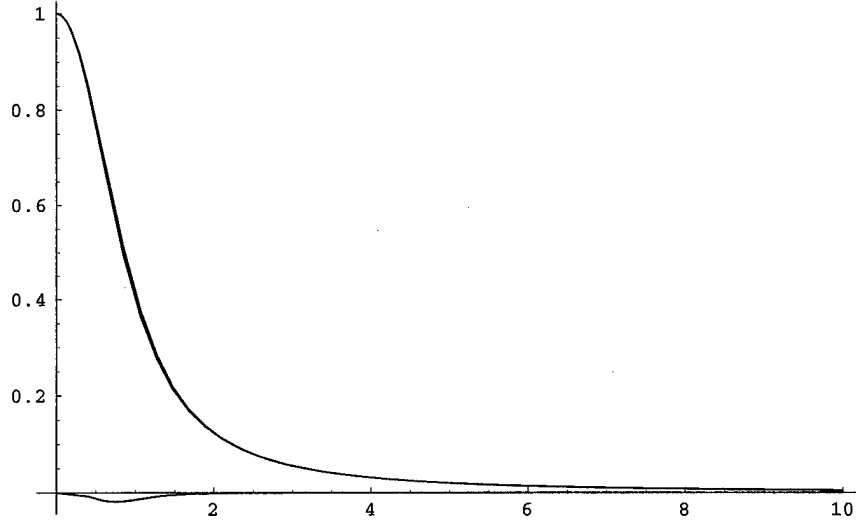
FIG. 6.1. Exact gain, its rational approximation (6.8) and their difference plotted as a function of \sqrt{p} . The approximation underestimates the exact value only slightly, by less than 3.5 percent.
