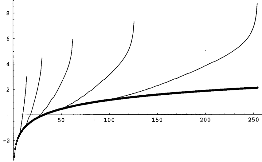
FIG. 5.3. Logarithm (base 10) of the numerical eigenvalues computed at various resolutions (thin lines, N = 17, 33, 65, 129, 257 ) and the analytic eigenvalues (thick dots). Increasing the number of points helps delay resolution failure, which still limits the number of correctly computed eigenvalues.
