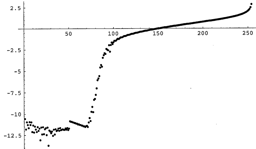
FIG. 5.2. Comparison of numerical and analytic eigenvalues for R = 100 and k = 0 . Logarithm (base 10) of the relative error is plotted. Virtually full machine accuracy is obtained up to the point of eigenfunction resolution failure near the 92nd eigenvalue. Chebyshev discretization of 257 points in the \rho direction was used.
