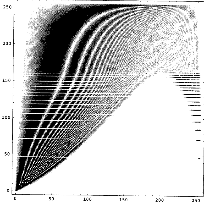
FIG. 5.4. Plot density shows magnitude of numerically obtained modes from the least stable (top) to the most stable (bottom) for the circumferential wavenumber k = 1 , using Chebyshev discretization in the \rho direction. There are 257 grid points from the cylinder wall at r = 1 (left) to the limit of the computational domain at r = 100 (right). The top portion is physically correct. Lower modes are numerical artifacts traced to the resolution failure starting near the gridpoint 200 of the eigenfunction shown at vertical coordinate 165, which corresponds to the 92nd eigenvalue.
