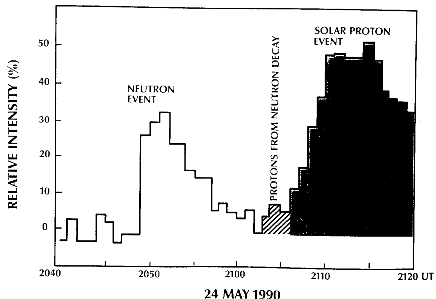
Figure 17. The identification of three components of solar flares by the Phillip's Laboratory's Geophysics Directorate will help predict solar particle events and protect Air Force space assets. Figure 17 charts the relative intensity of the three components of solar particles during a solar flare.
