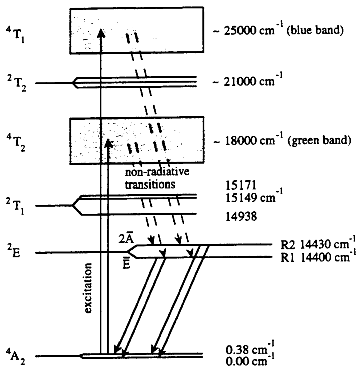
Fig. 1. Low-lying electronic levels of \text{Cr}^{3+} in sapphire, designated by their representations in the cubic-field terms ( O_h group) on the left. Fine structures, labeled on the right-hand side, result from the trigonal-field distortion of the corundum lattice and spin-orbit interactions. Splitting of the ground state, {}^4A_2 , is too small to be resolved in the R-line optical spectra at room temperature.
