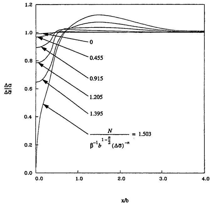
Fig. 4. The distribution of normalized stress in the band for several number of cycles, \beta b^{(n/2)-1} (\Delta \bar{\sigma})^n N , where the average initial damage level \omega_{\text{average}} = 0.01 , excess of damage in the band \omega_{\text{max}} - \omega_{\text{average}} = 0.09 , normalized size of the damage cluster 2\lambda = 1 , power n = 2 , and b is the average spacing between microcracks.
