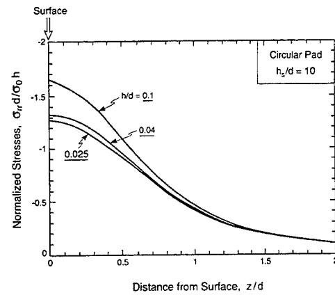
Fig. 10. Stresses in the substrate beneath a circular pad, at the symmetry location ( y = 0 ): (a) thin substrate, h_s/d = 1 ; (b) thick substrate, ( h_s/d = 10 ).
