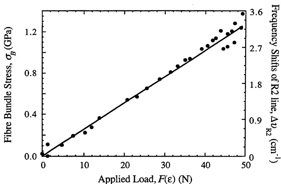
Figure 5. A typical load–stress curve for Nextel 610 fibre bundle. Here the bundle stress is deconvoluted from the average frequency shift using equation (2.8). The slope of the line corresponds to the overall cross-section of the initial load carrying fibres. Based on the average fibre diameter ( 12.06\ \mu\text{m} ), the number of initial load carrying fibre is 339 in this particular case, about 90% of the 377 fibres in the tow.
