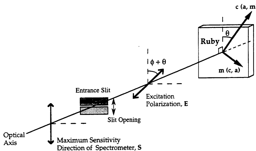
Fig. 2. Schematic diagram of the optical backscattering arrangement used in the fluorescence measurements. Direction of maximum sensitivity of the spectrometer, S , the slit configuration and opening direction, and the optic axis are indicated, as well as the polarization direction of the light used to excite the fluorescence. Notation c(a, m) denotes the orientation of the ruby crystallographic axes in successive experiments.
