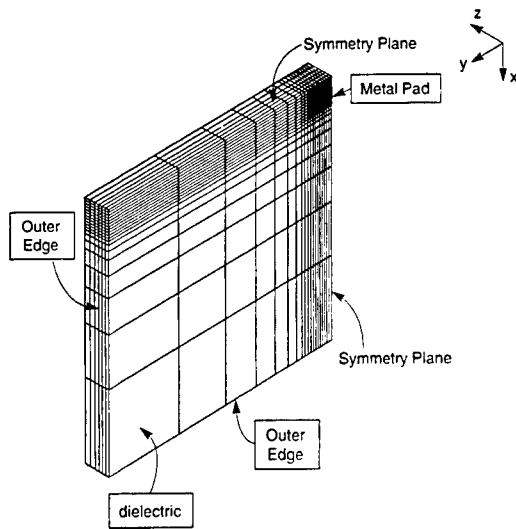
Fig. 12. The finite element mesh used for analysis of the square pad. For symmetry reasons, only 1/4 of the pad/substructure need be analyzed. The metal pad is at the top right outlined by ABCD. It is located on the face projected onto the plane of the figure.
