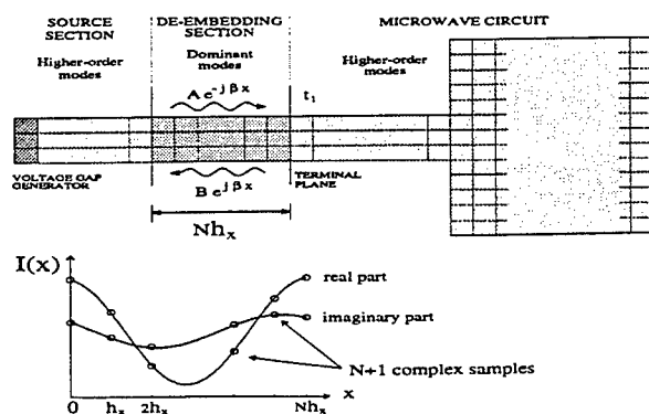
Fig. 2. De-embedding section.
