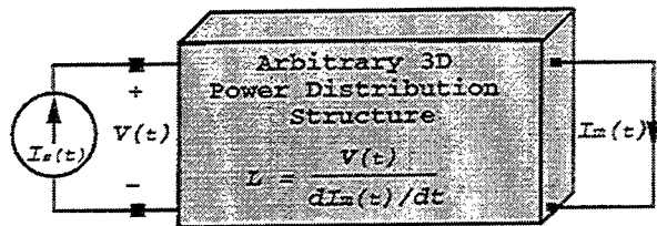
Figure 6: Power distribution structure.
