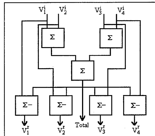
Figure 3 - Block Diagram of the TLM Processing Element
