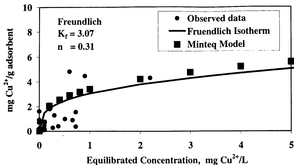
Figure 4-14: Copper adsorption isotherm obtained with Supelcarb™. Minteq model results plotted as dark square.
