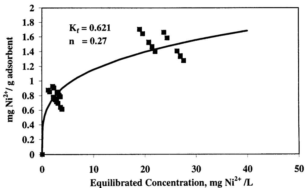
Figure 4-9: Nickel adsorption isotherm obtained with Carboxen-1011 TM in the batch experiments.
