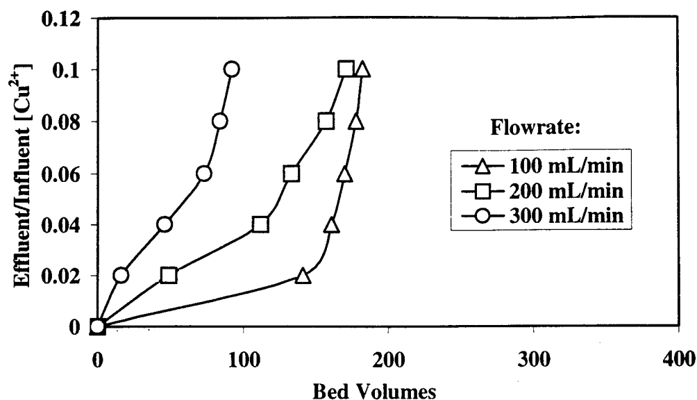
Figure 4-6: Copper breakthrough curves obtained with Carboxen-1011 TM and a constant influent concentration of 5 mg \text{Cu}^{2+} /L in the flow through experiments. Error bars represent a standard deviation about a triplicate mean.
