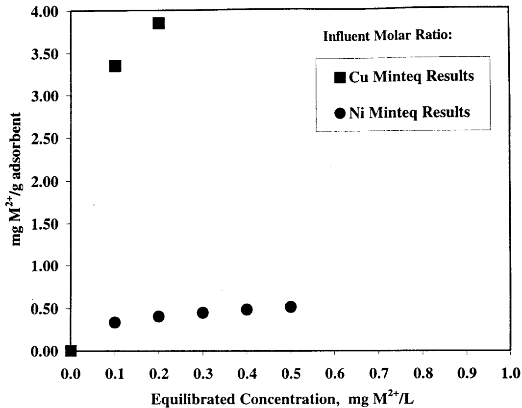
Figure 4-19: Minteq model of of a combined Ni^{2+} and Cu^{2+} batch adsorption experiment with Carboxen-1011 TM . Minteq simply super-positioned the adsorption isotherms for each metal. This result is caused by Minteq's assumption of infinite adsorption sites on the charred porous polymers.
