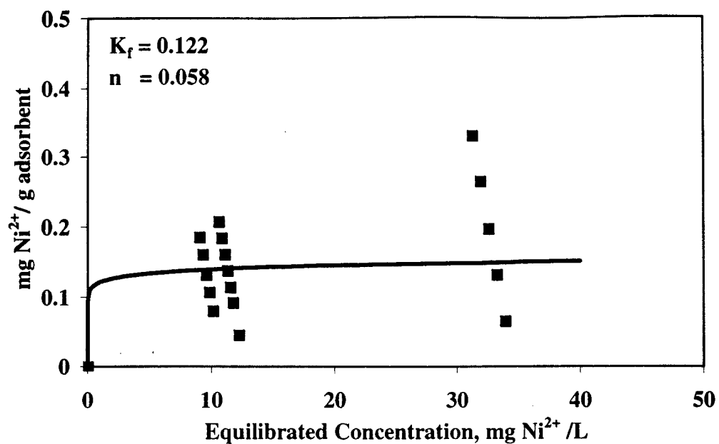
Figure 4-8: Nickel adsorption isotherm obtained with Supelcarb TM in the batch experiments.
