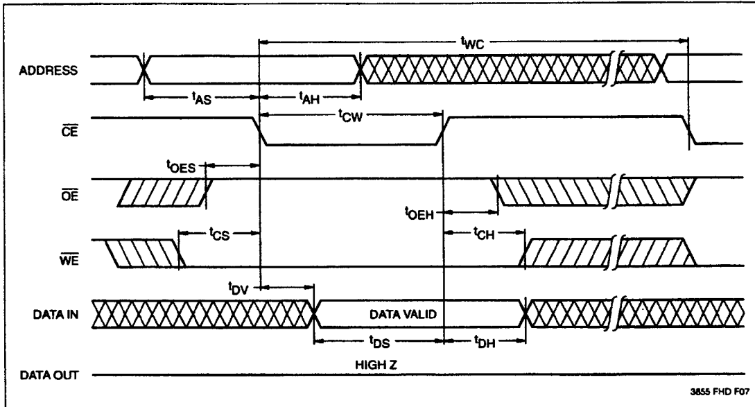
CE Controlled Write Cycle
