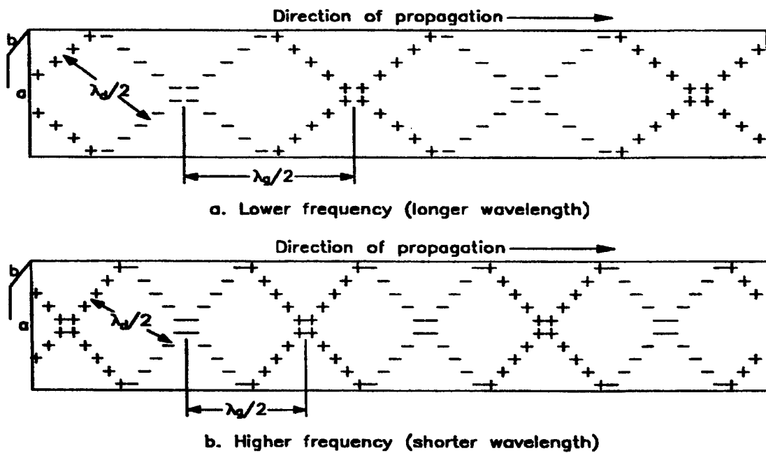
Figure 6.5: TE_{10} propagation electric fields.
