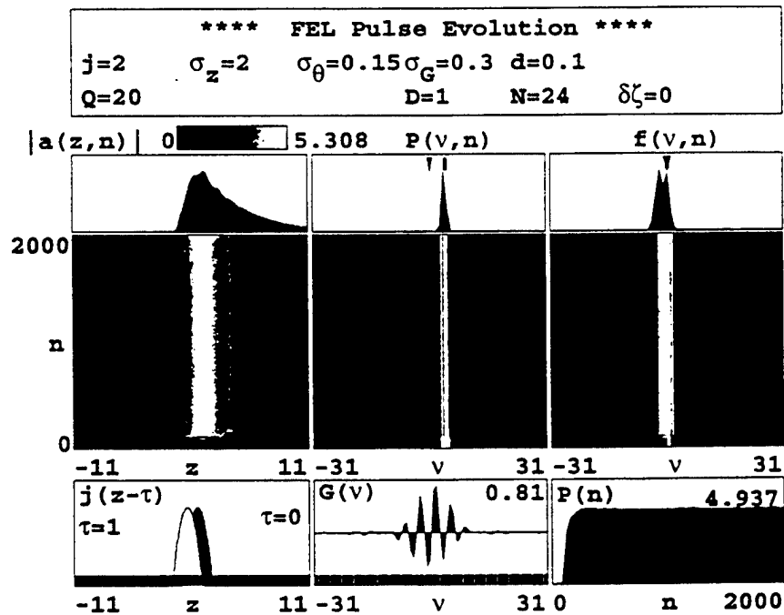
Figure 18. Pulse evolution for D = 1 and d = 0.1 .
