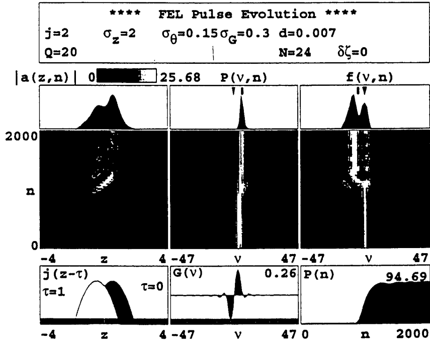
Figure 14. Pulse evolution for D = 0 at d = 0.007 .
