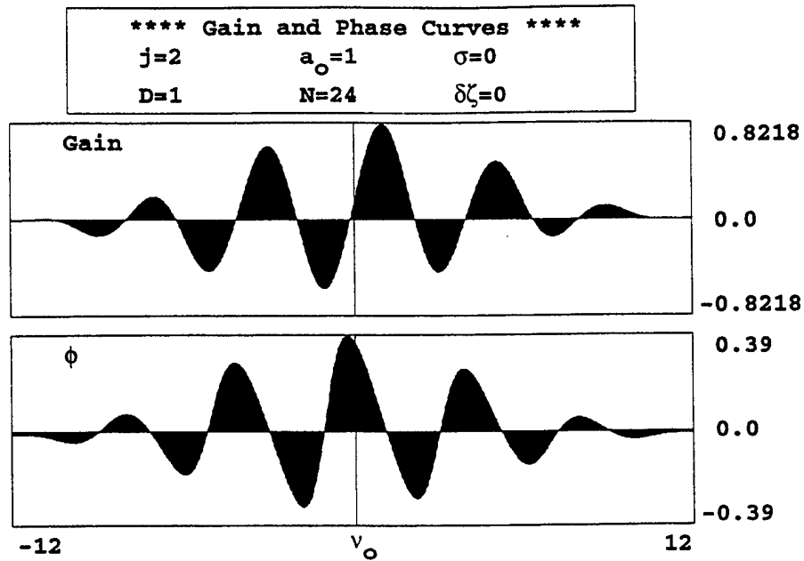
Figure 12. Gain spectrum for a low-current, weak-field optical klystron FEL.
