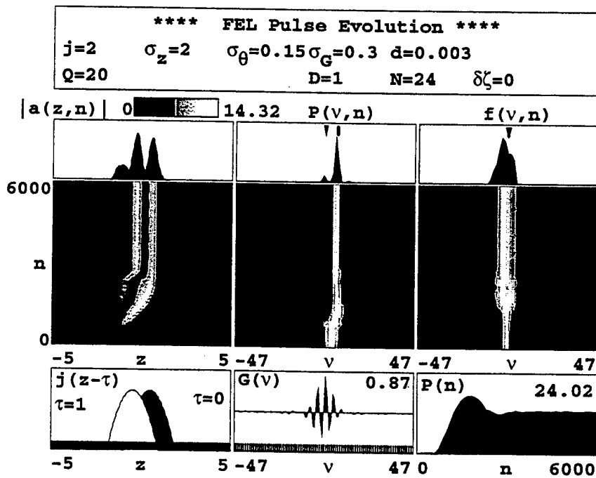
Figure 17. Pulse evolution for D = 1 at d = 0.003 .
