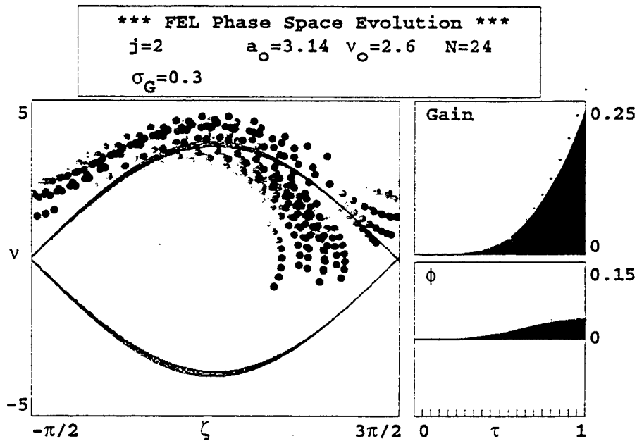
Figure 2. Phase space diagram.
