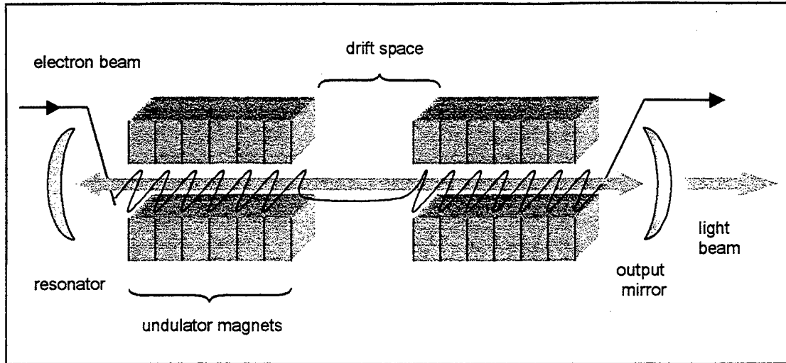
Figure 11. Optical klystron undulator with drift space.
