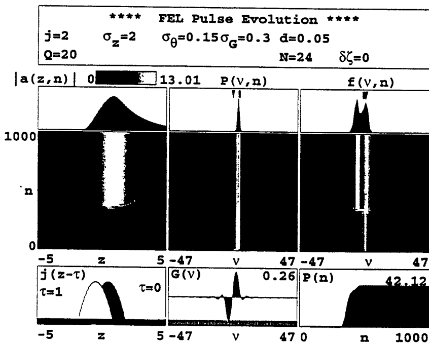
Figure 15. Pulse evolution for D = 0 at d = 0.05 .
