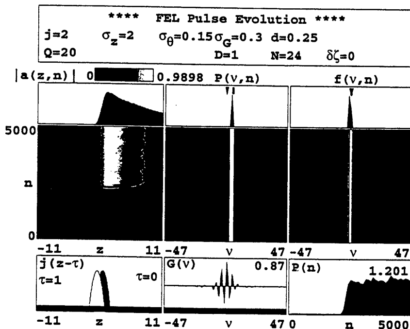
Figure 19. Pulse evolution for D = 1 at d = 0.25 .
