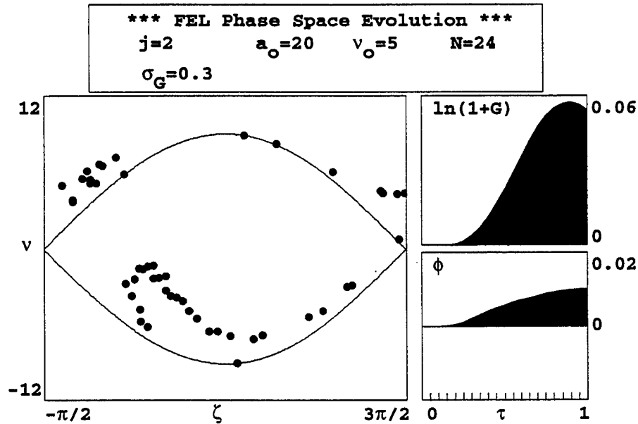
Figure 7. Strong-field phase space evolution with low current.
