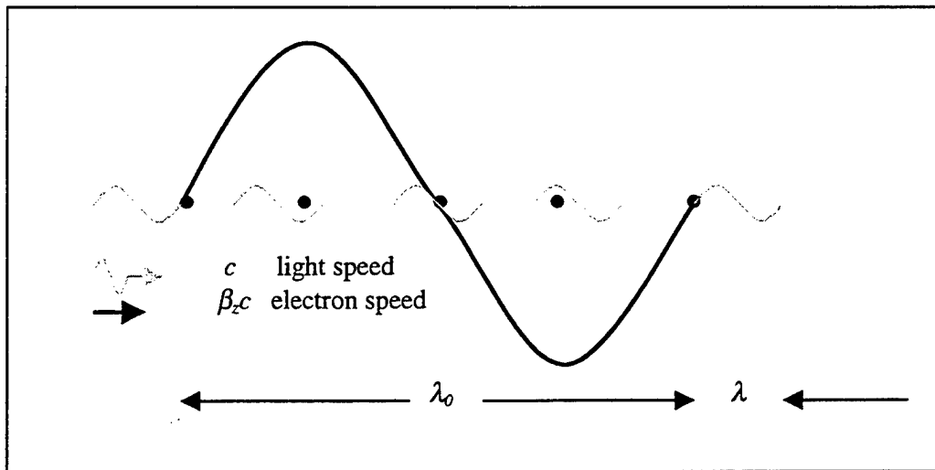
Figure 3. FEL resonance.
