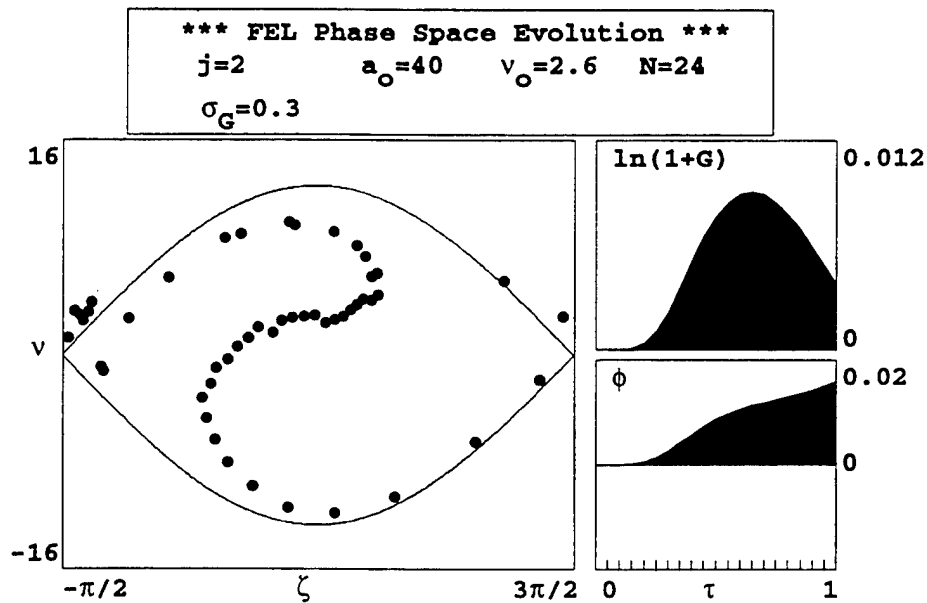
Figure 13. Phase space evolution demonstrating trapped-particle instability. sufficient for trapped-particle instability and a full synchrotron oscillation of the electrons. As the electrons bunch in strong optical fields, the electrons pass through the optimal phase for bunching, \zeta + \phi \approx \pi , and overbunch as they are trapped in the potential wells due to the strong optical field. This overbunching causes saturation and a decrease in the final gain.
