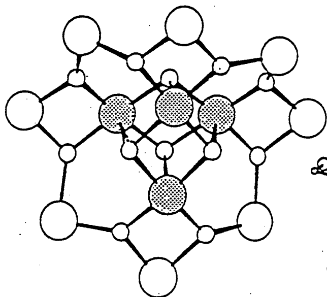
Schematic view of the core of a [\text{Mn}_{12}\text{O}_{12}(\text{carboxylato})_{16}] cluster in which only the metal atoms and the bridging oxygen atoms (small circles) are shown. The manganese(IV) atoms are enhanced by the shadowing.
