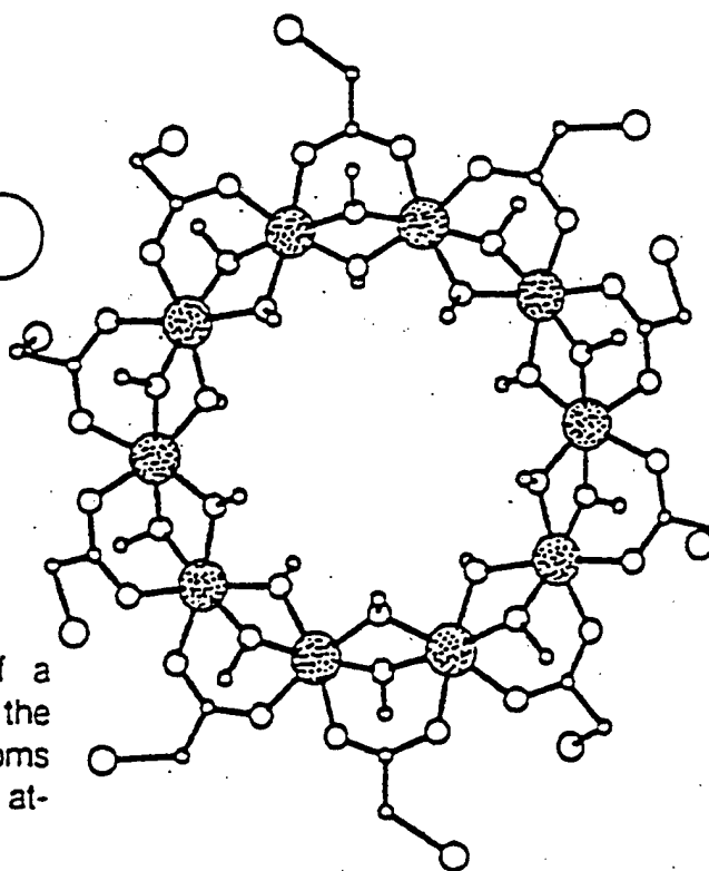
View of the ring structure of the \text{Fe}_{10} cluster, where the dotted circles represent the iron atoms and the empty circles are, in order of decreasing size, chlorine, oxygen, and carbon.
