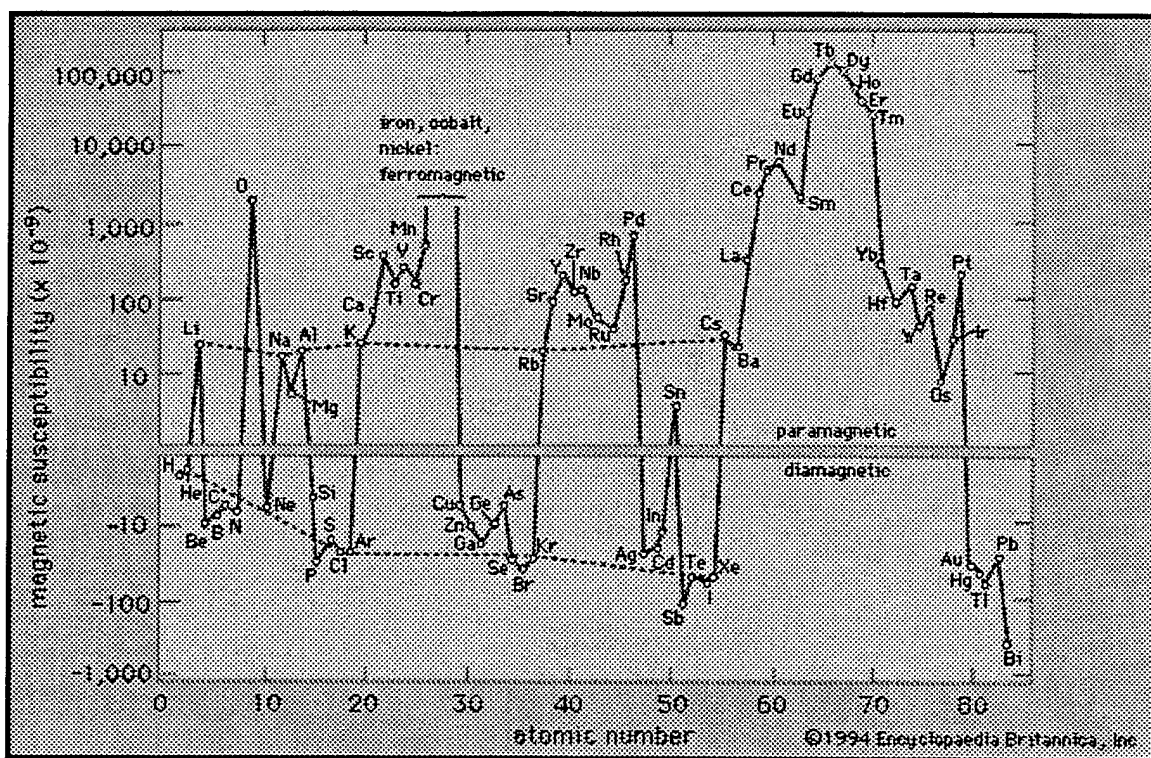
Figure 2. Diamagnetic elements in lower portion, paramagnetic in upper [From Ref. 27]
