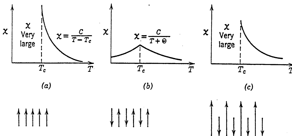
Figure 4. Magnetic susceptibility versus T for (a) ferromagnetic, (b) antiferromagnetic, and (c) ferrimagnetic materials, with magnetic moment alignments indicated for each case. [After Ref. 1]
