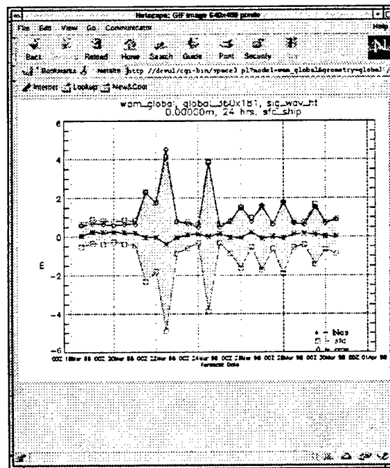
Figure 13. WAM_GLOBAL Statistics Graph
