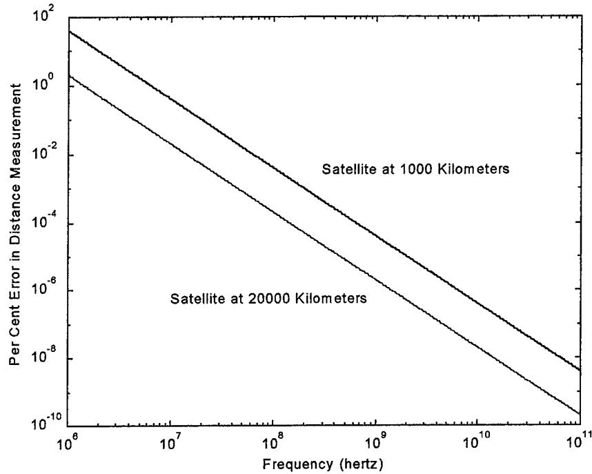
Figure 64. Distance measurement errors from two satellites
