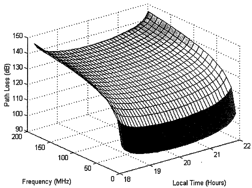
Figure 44. Path loss for example values.
