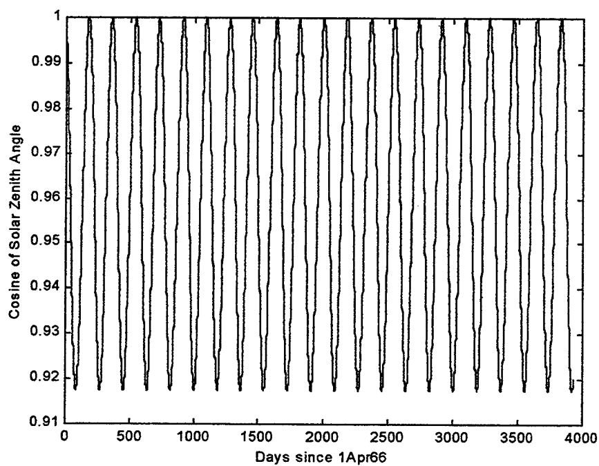
Figure 21. Cosine solar zenith angle.
