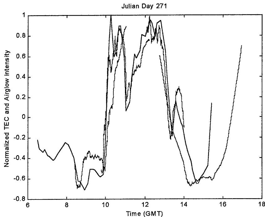
Figure 84. Normalized Airglow and TEC during TEP.
