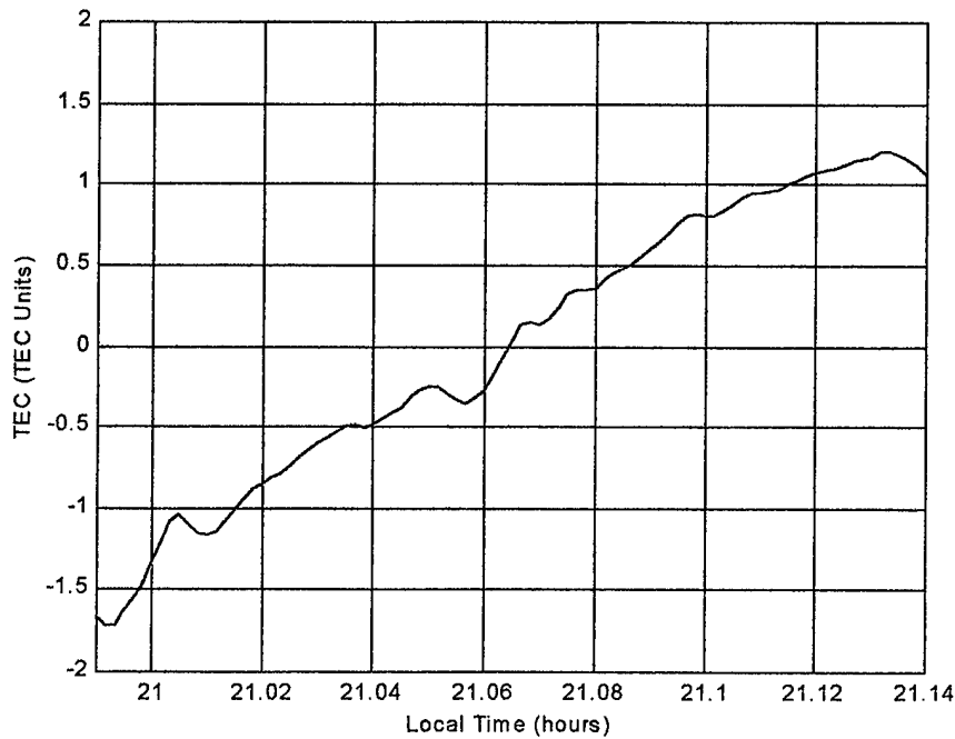
Figure 65. Change in TEC with change in time
