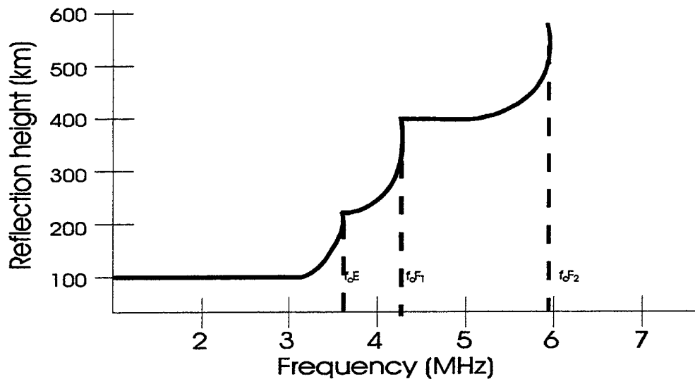
Figure 11. Ideal vertical incidence ionogram (After Hunsucker, 1991).
