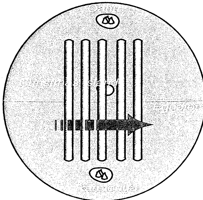
Figure 10. Ionospheric ducts moving eastward in nighttime sky
