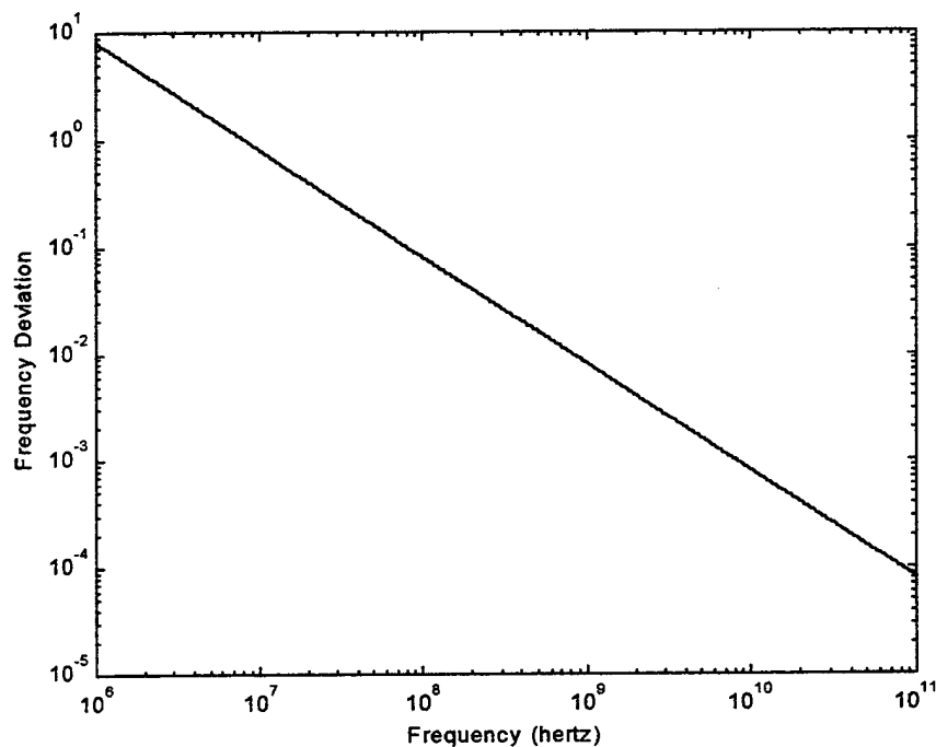
Figure 66. Frequency deviation caused by scintillation
