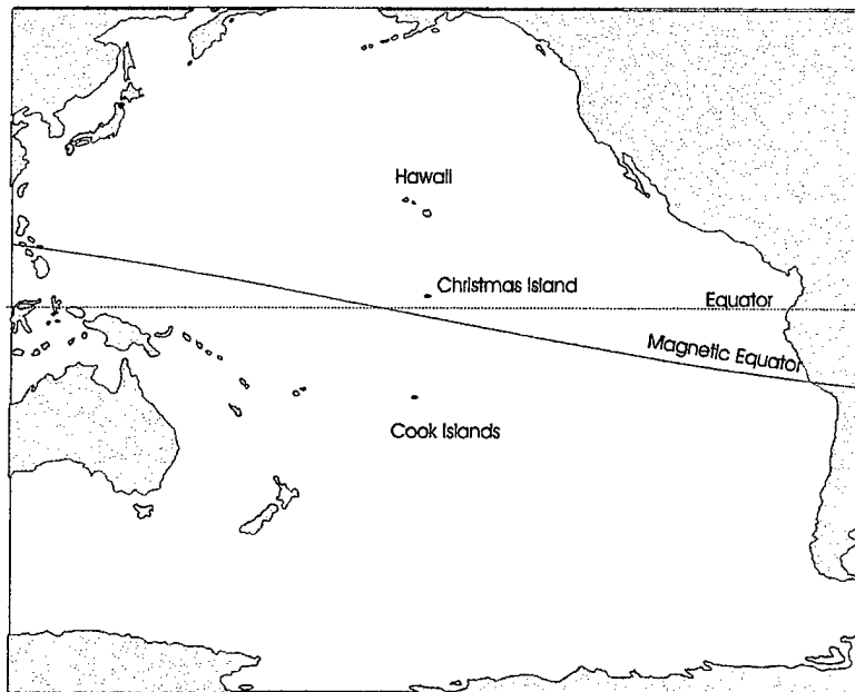
Figure 17. Central Pacific showing Hawaii, Cook Islands, and Christmas Island.
