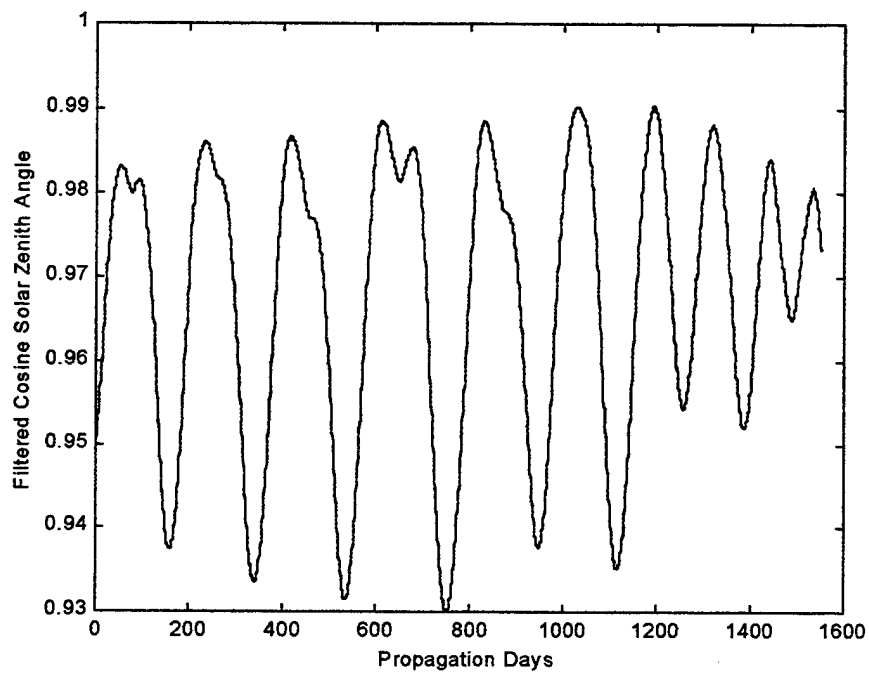
Figure 27. Filtered cosine solar zenith angle.
