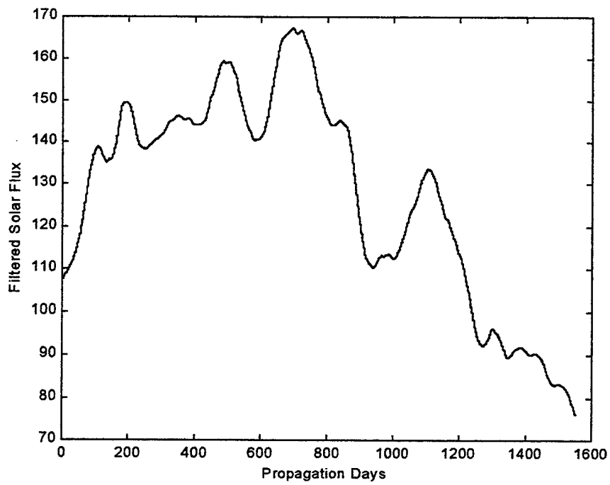
Figure 26. Filtered solar flux.
