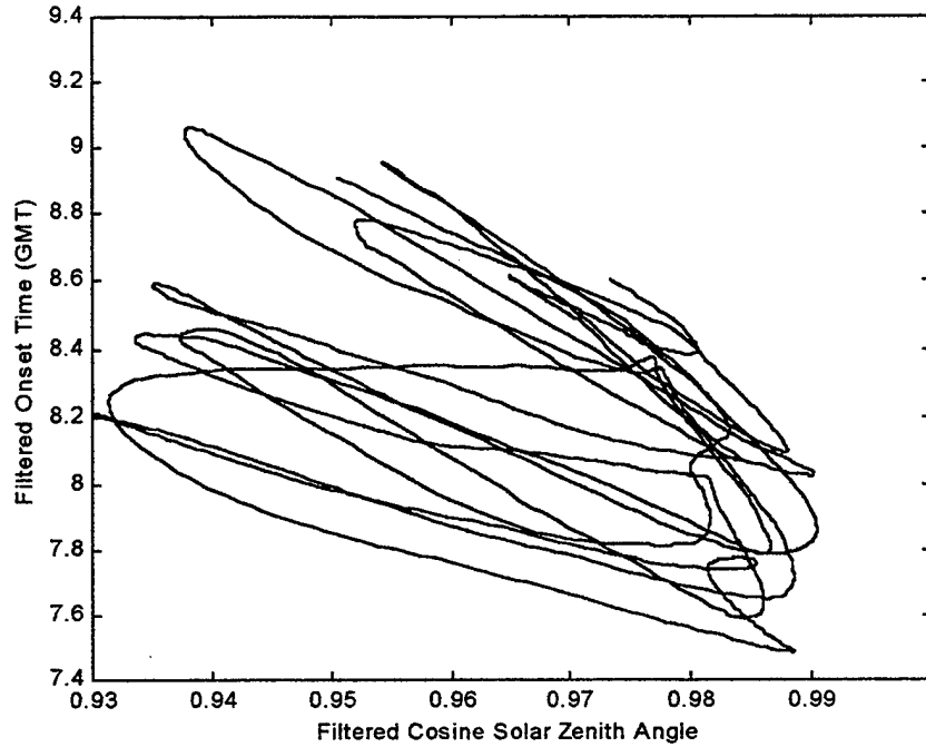
Figure 29. Filtered onset time versus filtered cosine solar zenith angle.
