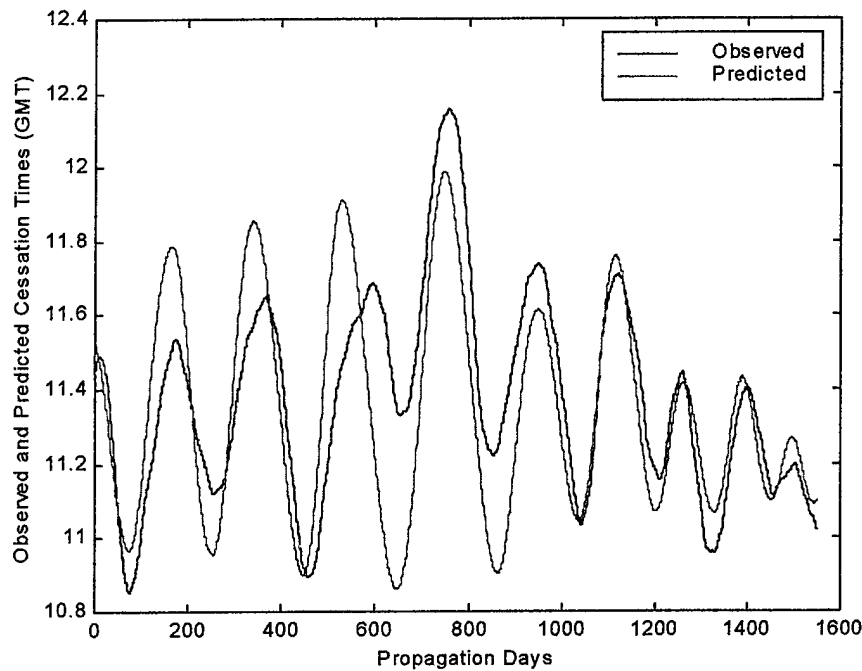
Figure 34. Comparison of observed and predicted cessation times.
