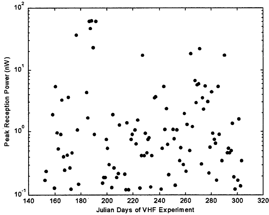
Figure 43. Peak daily reception power at Rarotonga.
