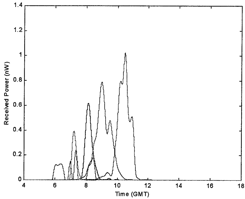
Figure 41. Signal strength roll-off with time over five days. Each day is represented by a different color.
