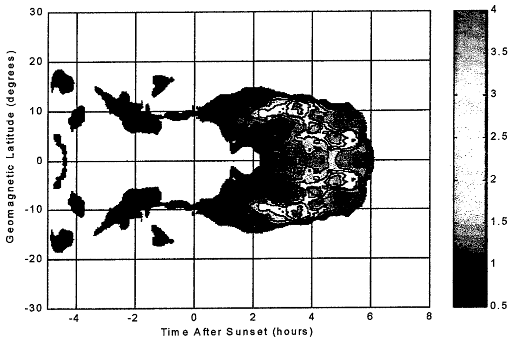
Figure 61. Scintillation standard deviation seen from above
