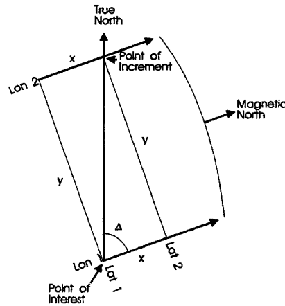
Figure 85 Computing the Magnetic Declination Angle
