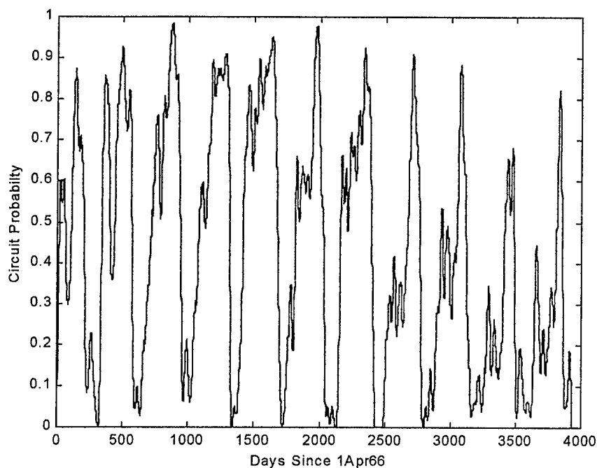
Figure 35. Twenty-one day moving average TEP circuit probability.
