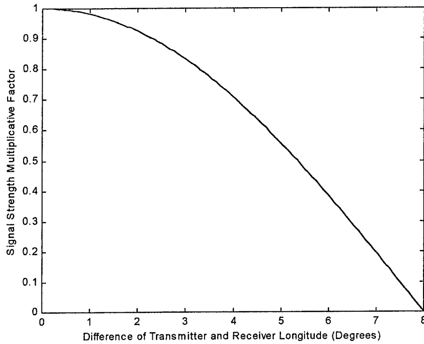
Figure 40. Longitudinal coupling factor.
