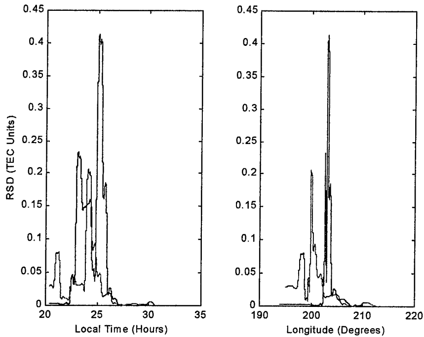
Figure 55. Running standard deviation for PRN 2 and PRN 4
