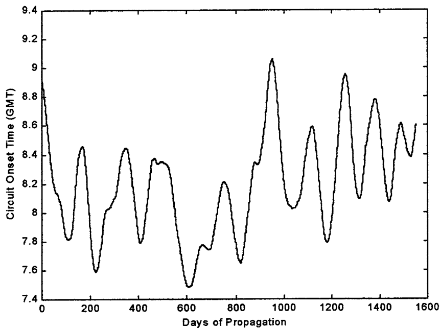
Figure 25. Filtered onset times.
