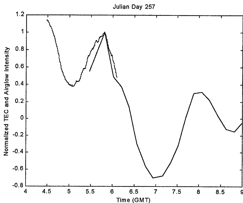
Figure 85. Normalized Airglow and TEC with no TEP.
