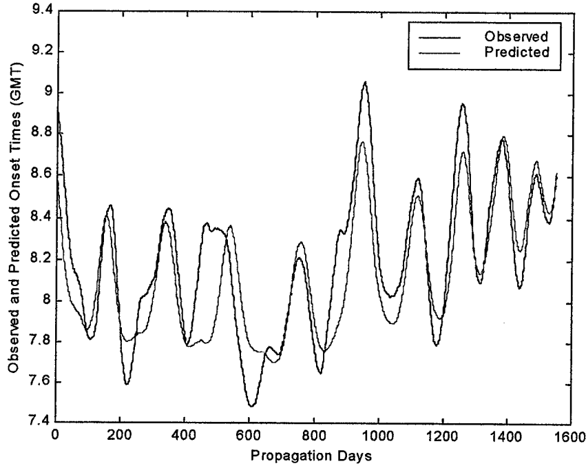
Figure 31. Observed and predicted onset times.
