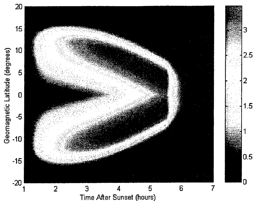
Figure 70. Scintillation prediction from above.
