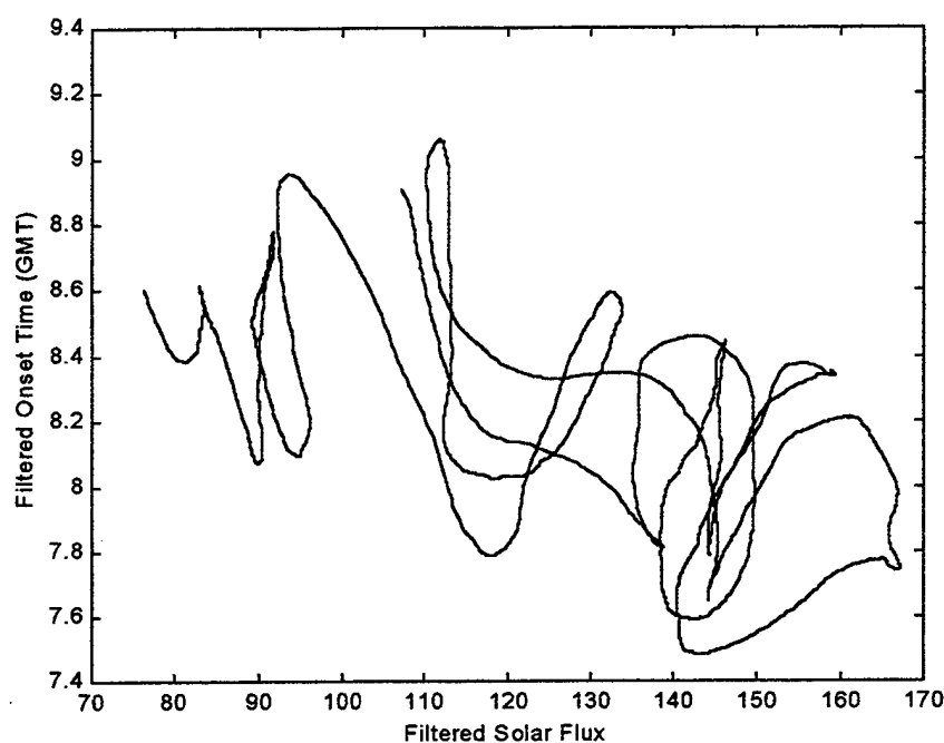
Figure 28. Filtered onset time versus filtered solar flux.
