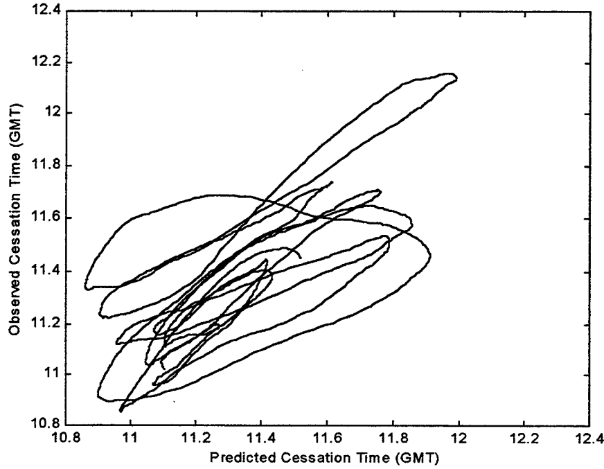
Figure 33. Observed versus predicted circuit cessation time.
