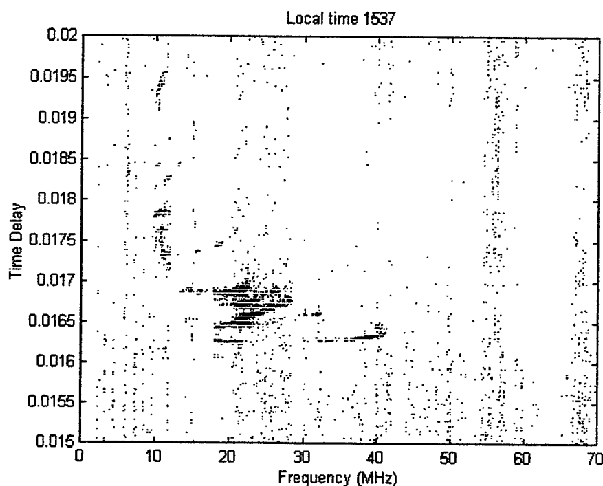
Figure 75. Emerging Afternoon-TEP at 1537.
