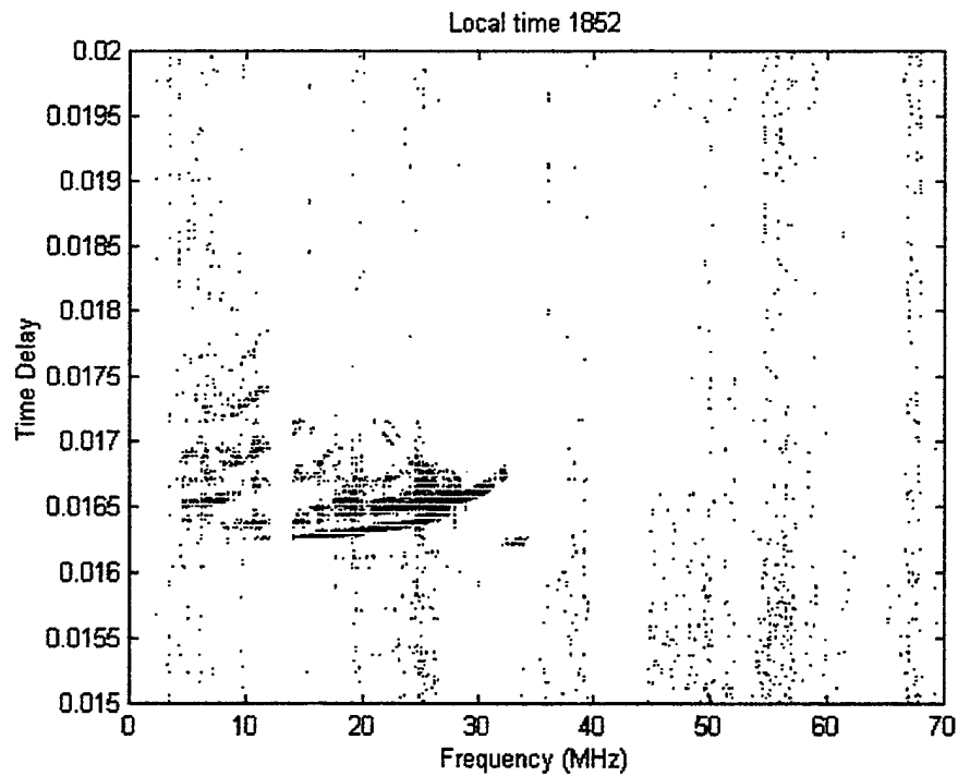
Figure 77. Afternoon-TEP trace disappears at 1852.
