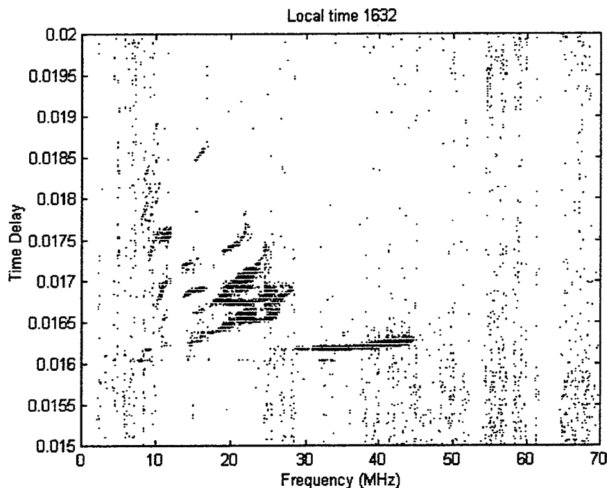
Figure 76. Afternoon-TEP extending to 46 MHz.
