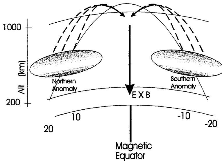
Figure 5. Plasma migration from anomalies to equator.
