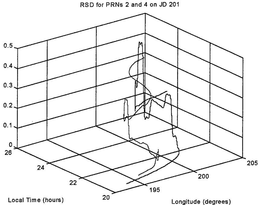
Figure 56. Running standard deviation plotted in three dimensions
