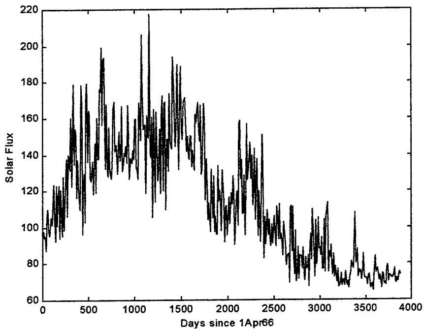
Figure 19. Solar flux.
