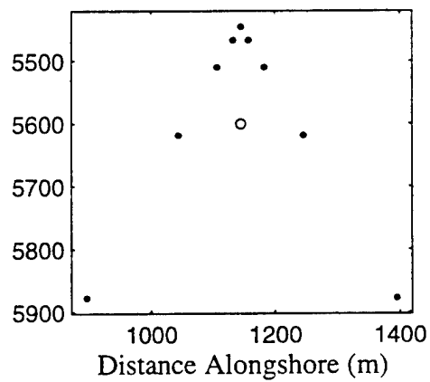
20 m Array and Buoy Sensor Locations
