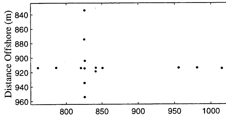
20 m Array and Buoy Sensor Locations
