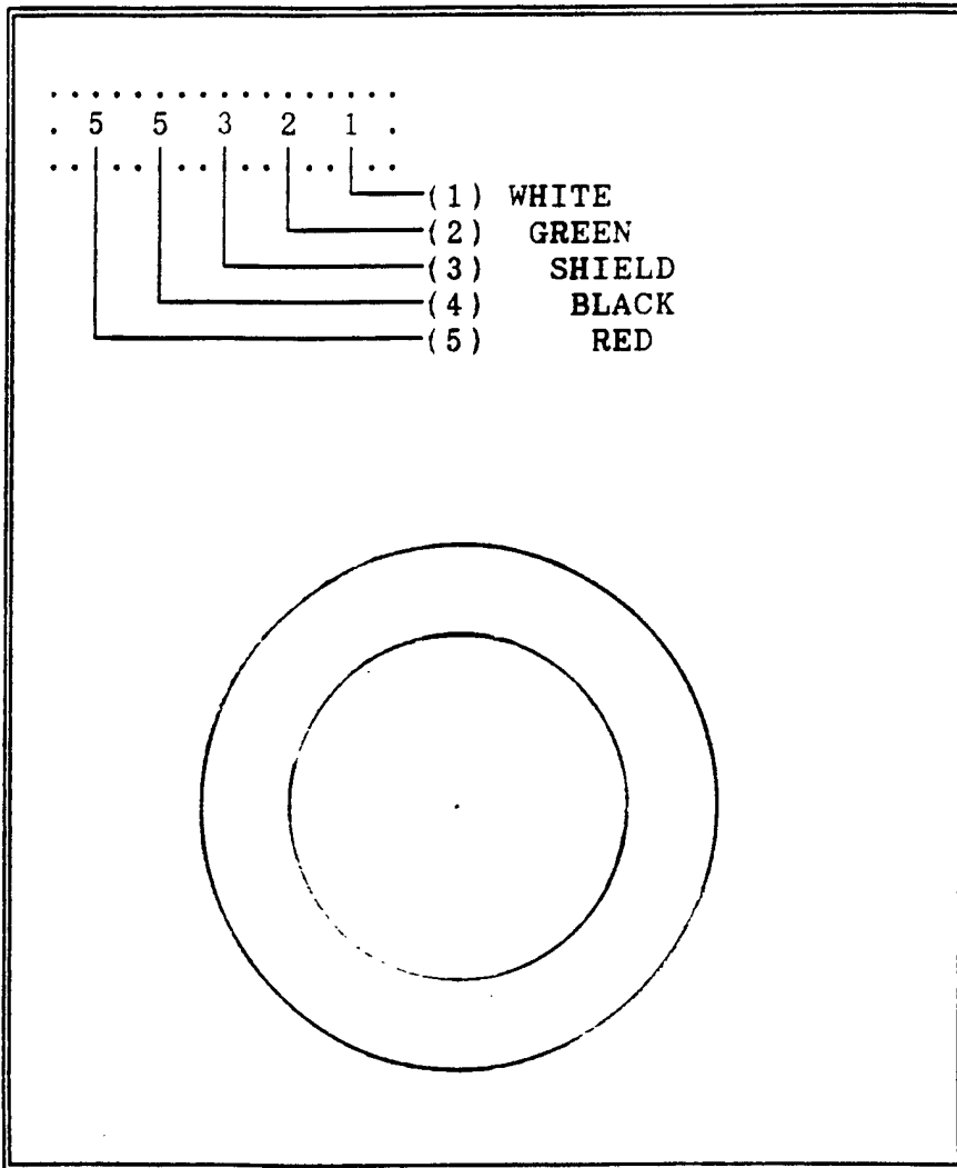
Current Sensor (Physical representation)
