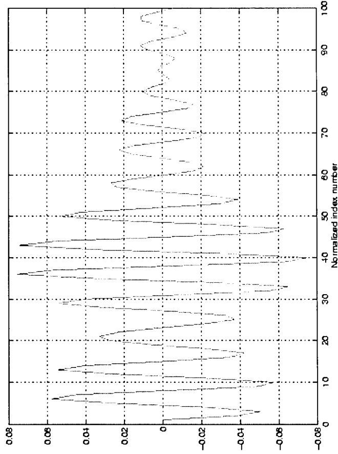
An eigenvector
