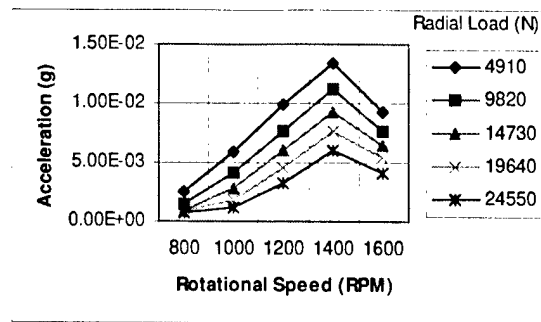
Fig. 2. 4-6 kHz Envelope Spectrum Peak, Z Accelerometer, Housing Top.
