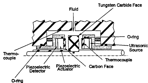
Figure 1. Apparatus
